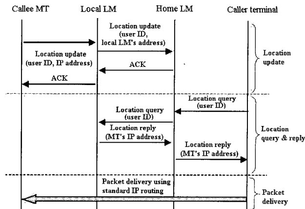
Fig. 4. Location update and query.
