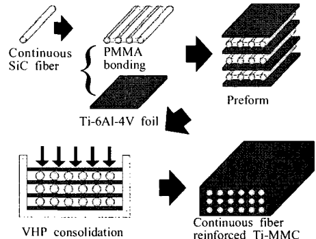
Fig. 2 Consolidation processes with SiC fiber and Ti-6Al-4V foil using FFF method.
