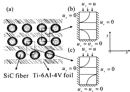
Fig. 6 Schematic diagrams showing (a) fiber and matrix arrays, (b) rectangular unit cell-model, and (c) triangular unit cell-model for FEM simulations.
