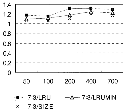
(Fig. 8) Gain ratio of object-hit on 7 : 3
