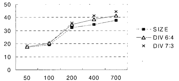
(Fig. 6) Object-hit ratio(%) : compared with SIZE
