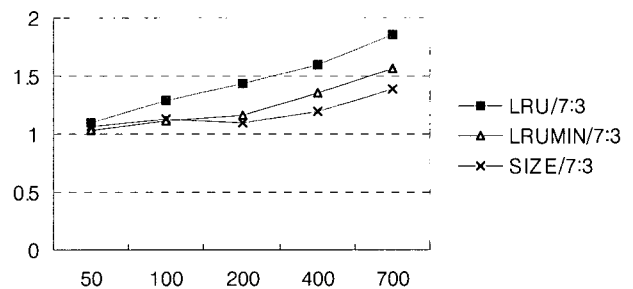
(Fig. 10) Gain ratio of response time on 7 : 3
