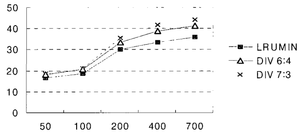
(Fig. 5) Object-hit ratio(%) : compared with LRU-MIN
