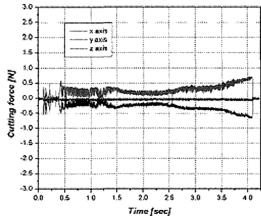
Fig.15 Normal cutting force ( V=900 mm/min, cutting depth 5 \mu\text{m} /pass, Tool R600 \mu\text{m} , Ni)
