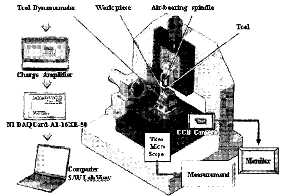
Fig. 3 Micro machining system and schematic of experimental system
