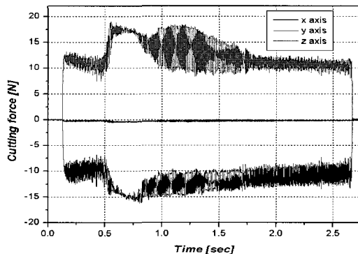
Fig.16 Excessive cutting force ( V=900 mm/min, depth 5 \mu\text{m} /pass, Tool R600 \mu\text{m} , Ni)
