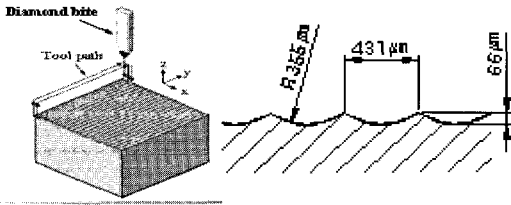
Fig. 5 Machining method and scheme of lenticular lens
