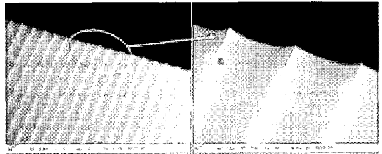
Fig. 7 Machining result of cutting speed 900 mm/min
