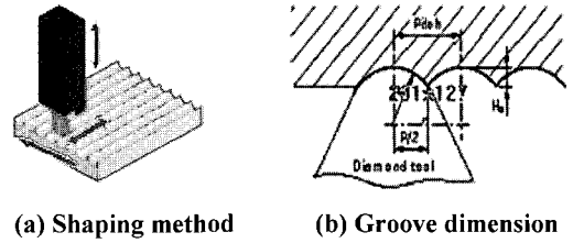
Fig. 2 Machining method of lenticular lens mold
