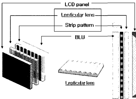
Fig. 1 Stereoscopic module and lenticular lens
