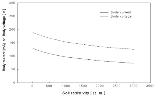
Fig. 4. Body current and body voltage by the graphical method.
