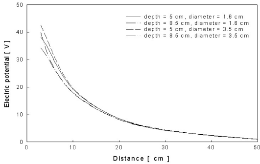
Fig. 14. Electric potential vs. distance from a street –lamp control –box source at 220 [V].
