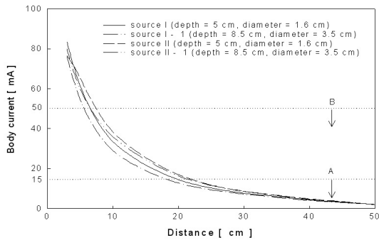
Fig. 17. Body current vs. distance at 220 [V].
