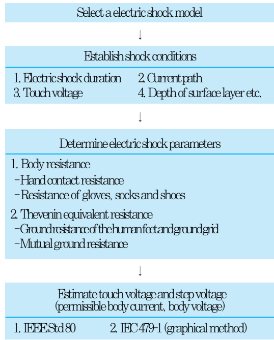
Fig. 1. Block diagram for hazard assessment of the electric shock.
