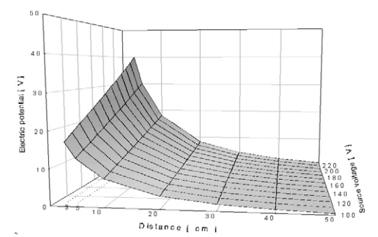
Fig. 12. Electric potential with a street-lamp control box source II-1 in case of submerged depth=8.5 [cm] and rod diameter=3.5 [cm].
