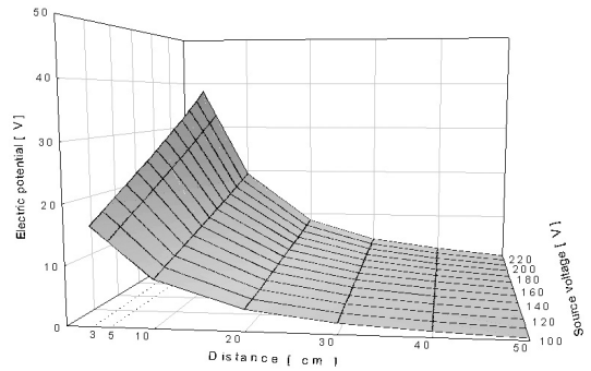
Fig. 11. Electric potential with a street-lamp control box source II in case of submerged depth=5 [cm] and rod diameter=1.6 [cm].
