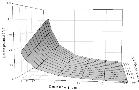
Fig. 9. Electric potential with a line source I in case of submerged depth=5 [cm] and rod diameter =1.6 [cm].
