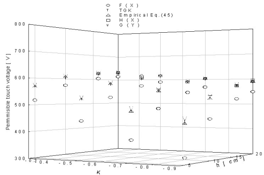
Fig. 6. Comparison of permissible touch voltage by IEC 479-1.
