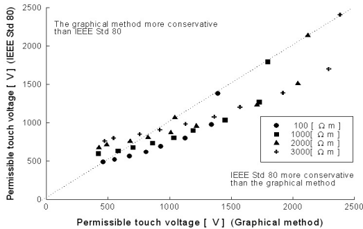
Fig. 3. Permissible touch voltages by the graphical method against IEEE Std 80, soil resistivity.
