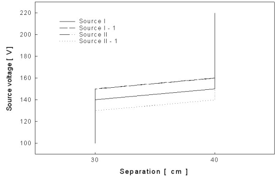
Fig. 16. Source voltage vs. separation in case of permissible touch voltage, 25 [V].
