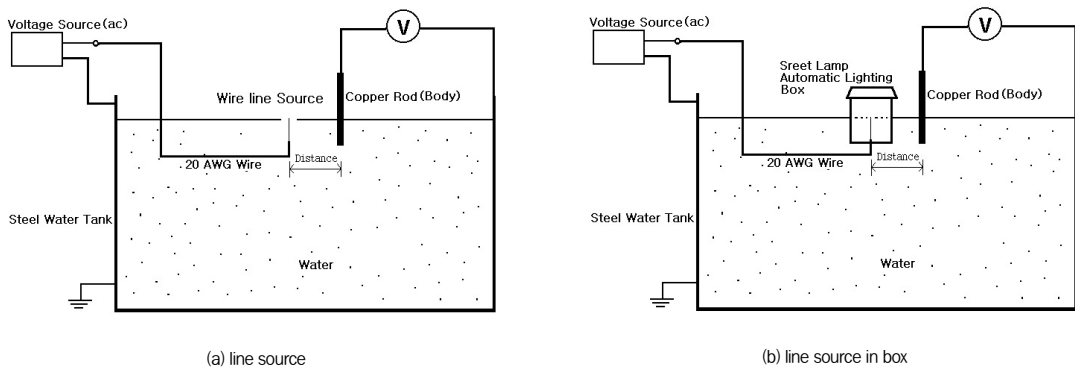
Fig. 2. Experimental setup for measurement of electric potential in fresh water.
