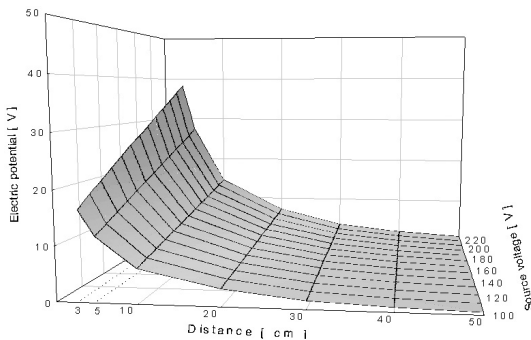
Fig. 10. Electric potential with a line source I-1 in case of submerged depth=8.5 [cm] and rod diameter =3.5 [cm].
