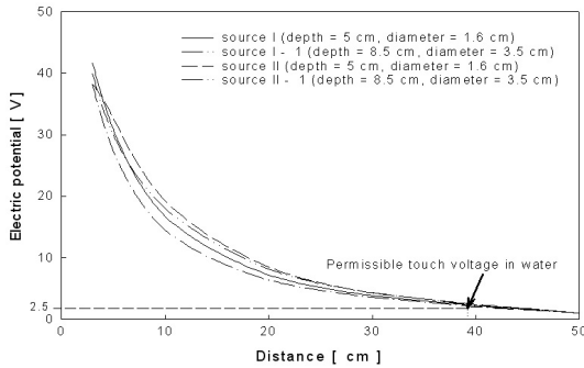
Fig. 15. Electric potential vs. distance at 220 [V].
