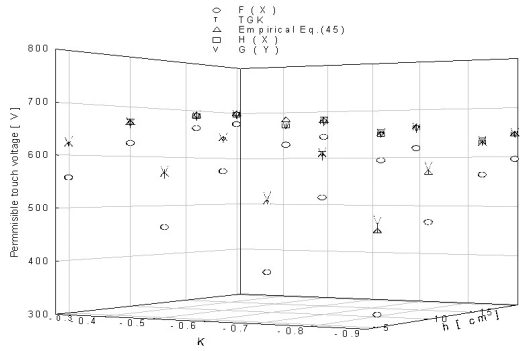
Fig. 5. Comparison of permissible touch voltages by IEEE Std 80.
