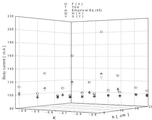
Fig. 7. Comparison of body current by IEC 479-1.
