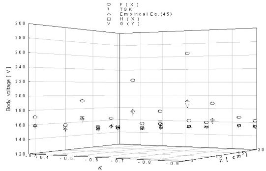
Fig. 8. Comparison of body voltage by IEC 479-1.
