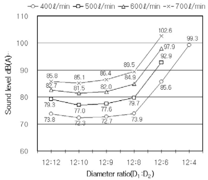
Fig. 5. Sound level on diameter ratio and air flow rate ( L_1:L_2=50:50 )
