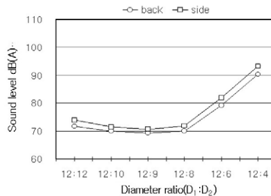
(b) distance=100cm, L_1:L_2=50:50 , Q=400 \ell / \text{min}
