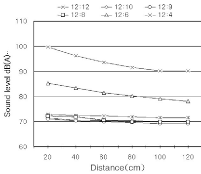
Fig. 7. Sound level on distance of between a reflection plate and a nozzle( L_1:L_2=50:50 , Q=400 \ell / \text{min} )
