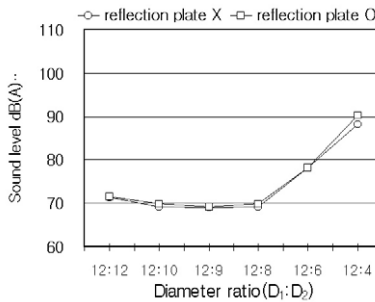
(c) distance=100cm, L 1 :L 2 =50:50, Q=400 l/min
