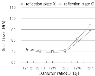
(b) distance=60cm, L 1 :L 2 =50:50, Q=400 l/min
