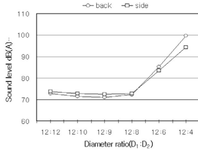
(a) distance=20cm, L_1:L_2=50:50 , Q=400 \ell / \text{min}
