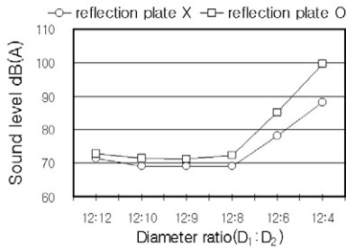
(a) distance=20cm, L 1 :L 2 =50:50, Q=400 l/min
