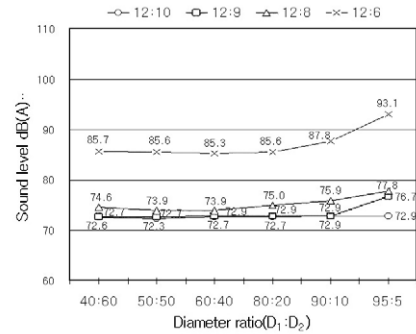
Fig. 6. Sound level on length ratio and diameter ratio ( Q=400 l/min)
