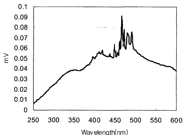
Fig. 1 Spectral intensity of light source.
