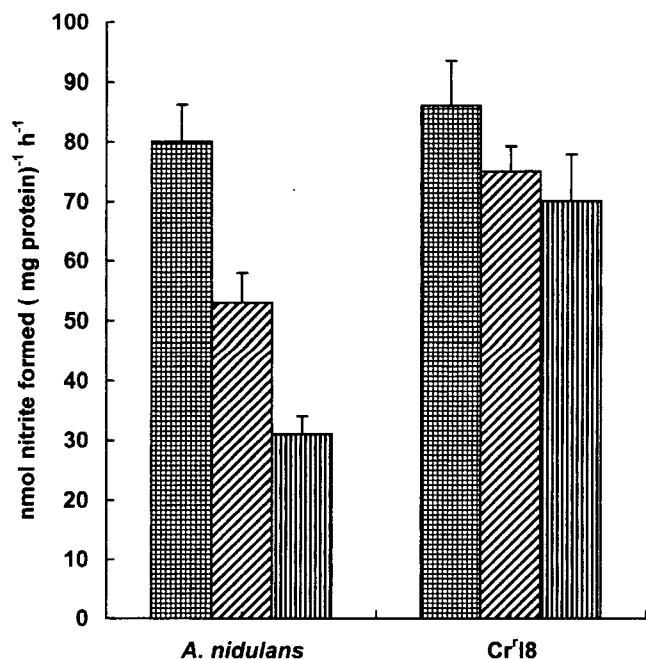
Fig. 2. NR activity in control (▣) and metal-supplemented ( 160 \mu\text{M Cr}^{6+} ) medium on 2 nd (▤) and 10 th (▥) d. 6-day-old cells were incubated in respective medium with 5 \text{ mM KNO}_3 . Values are mean \pm SD.
