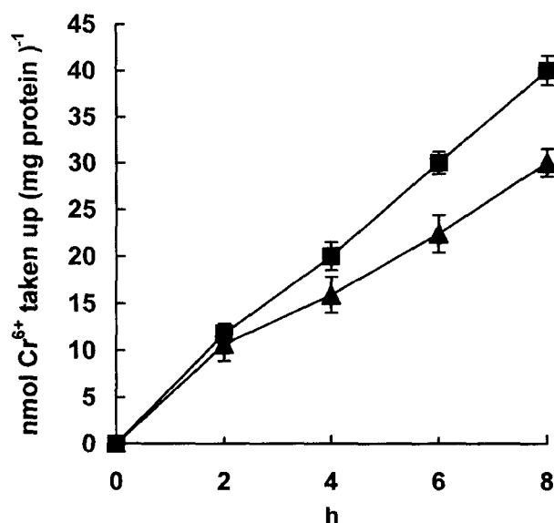
Fig. 4. Cr 6+ uptake by (150 µg protein ml -1 ) of A. nidulans (▲) and CrI8 (■) from Chu-10 medium (30 µM Cr 6+ ). Cells grown in medium devoid of Cr 6+ for 6 days were used for Cr 6+ uptake. Values are mean±SD.
