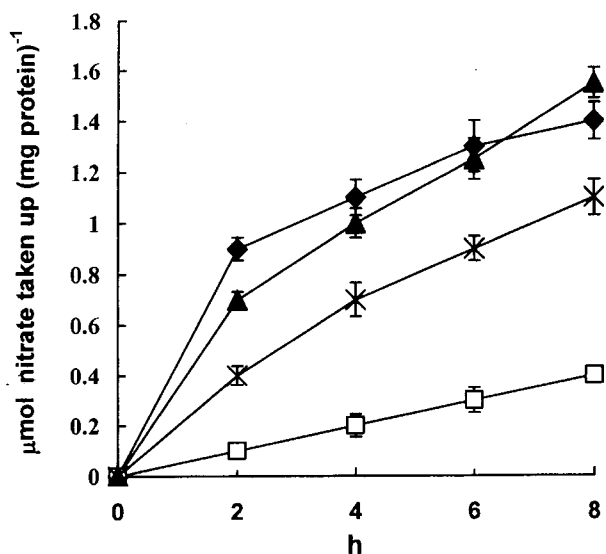
Fig. 1. Nitrate taken up from control medium (◆— A. nidulans , ▲—CrI8) and metal supplemented ( 160 \mu\text{M Cr}^{6+} ) medium (□— A. nidulans , ×—CrI8).
