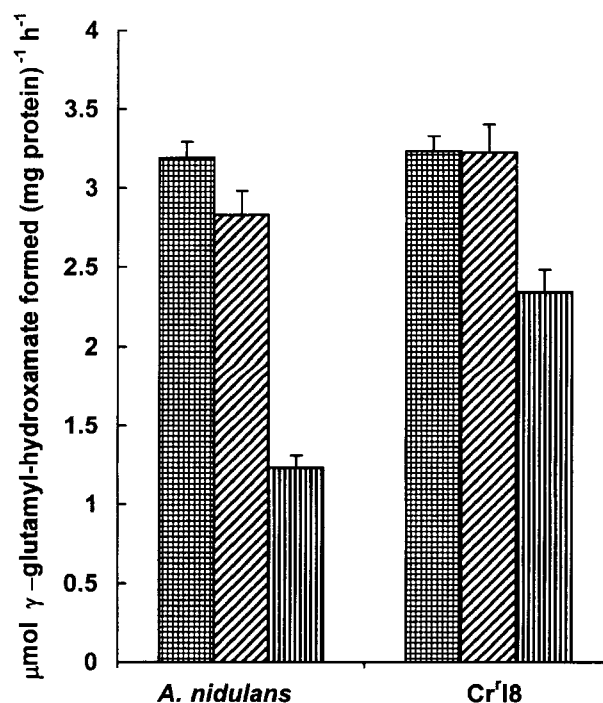
Fig. 3. GS activity in control (▣) and metal-supplemented ( 160 \mu\text{M Cr}^{6+} ) medium on 2 nd (▤) and 10 th (▥) d. Conditions were same as in Fig. 2. Values are mean \pm SD.
