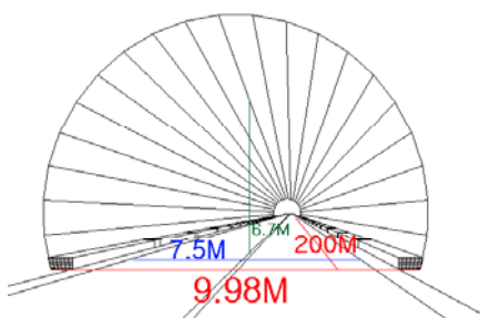
Figure 1. Tunnel structure
