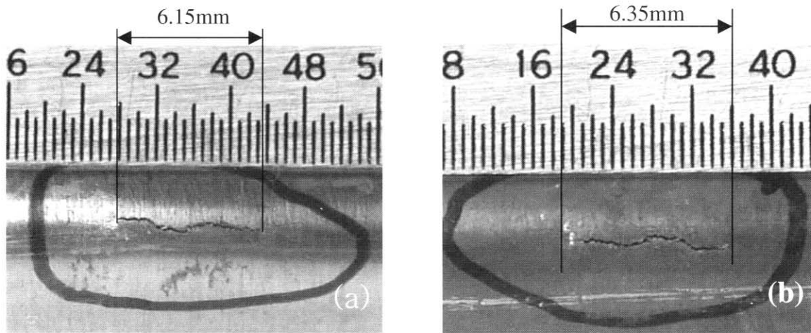
Fig. 5. Flaws on the SGH005 after (a) High temperature pressure test, (b) Room temperature pressure test.
