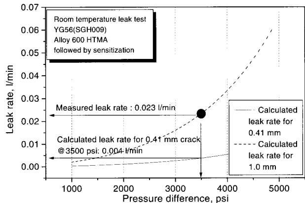
Fig. 7. Calculated and measured leak rate on the tube SGH009.
