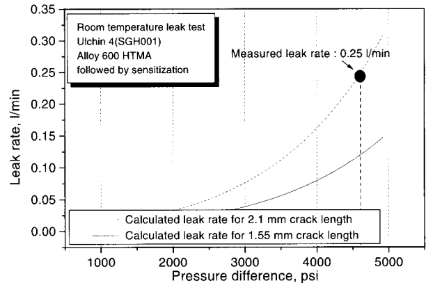
Fig. 6. Calculated and measured leak rate on the tube SGH001.
