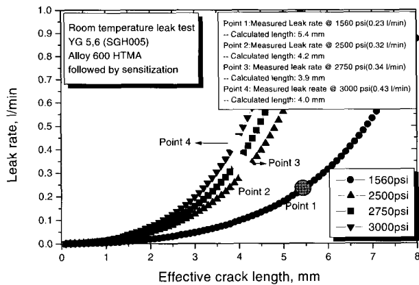
Fig. 11. Effective throughwall crack length on the tube YG5,6 calculated from the leak rate model (SGH006)
