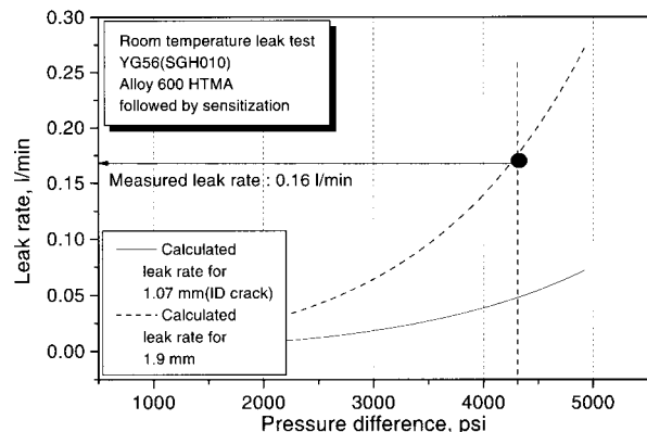
Fig. 8. Calculated and measured leak rate on the tube SGH010.
