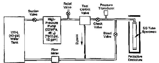
Fig. 1. Schematic of the pressure test facility.
