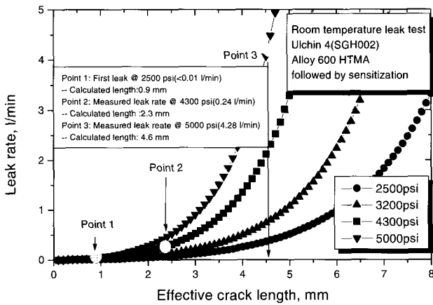
Fig. 9. Effective throughwall crack length on the tube Ulchin 4 calculated from the leak rate model (SGH002)
