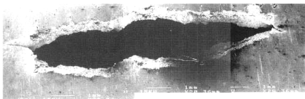
Fig. 2. Crack morphology of SGH002 after the pressure/leak test at room temperature.
