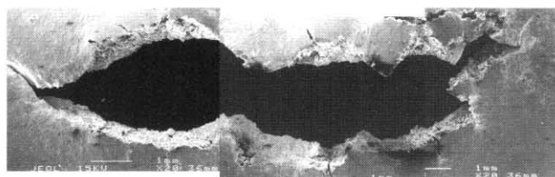
Fig. 3. Crack morphology of SGH006 after the pressure/leak test at room temperature
