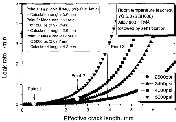
Fig. 10. Effective throughwall crack length on the tube YG5,6 calculated from the leak rate model (SGH005)
