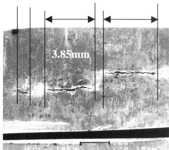
Fig. 4. Flaws on the SGH001 after the pressure/leak test at room temperature.
