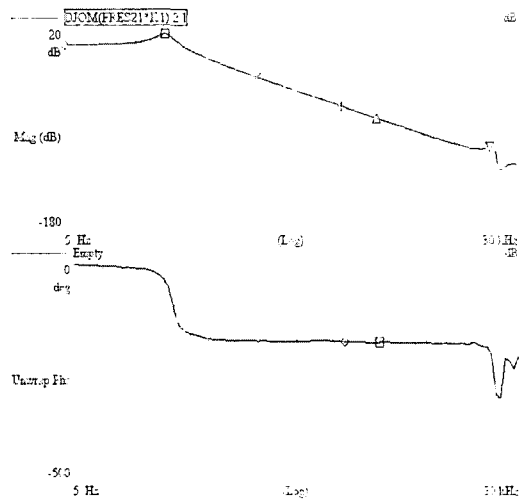
Fig. 6 Bode plot of PCB-Coil actuator (focus direction)
