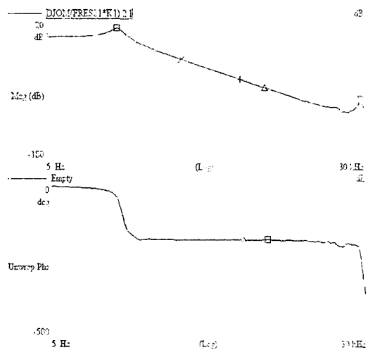
Fig. 7 Bode plot of PCB-Coil actuator (track direction)
