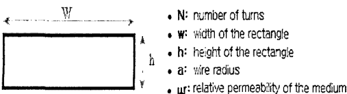
Fig. 5 Meaning of each factor for inductance
