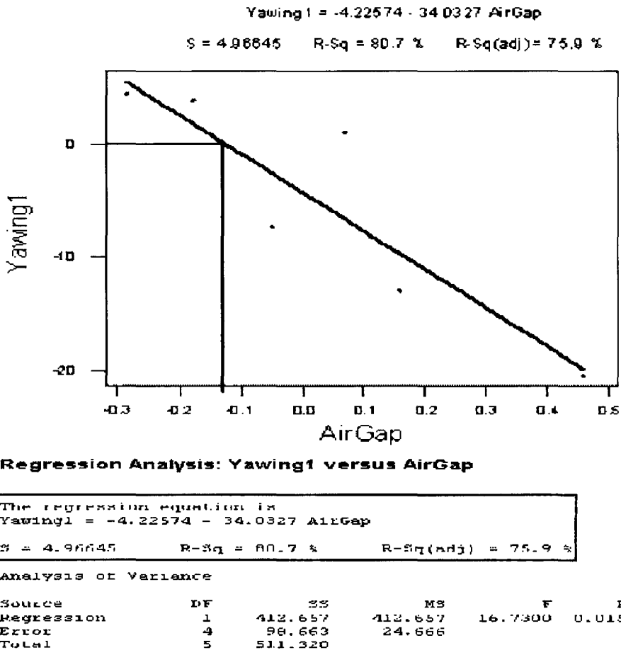
Fig. 2 Regression analysis of yawing and air gap
