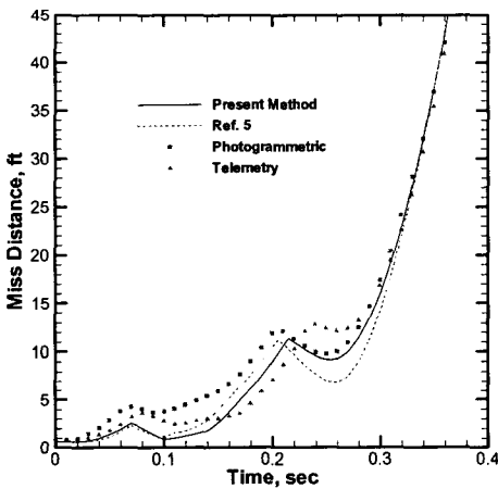
Fig. 9 Miss distance history (case 2)
