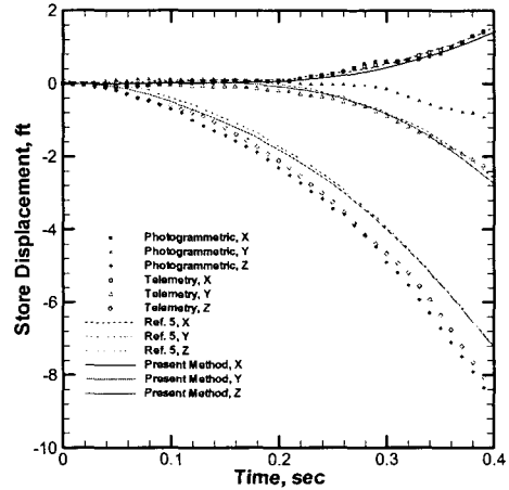
Fig. 3 Store displacement (case 1)
