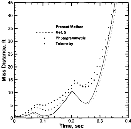
Fig. 8 Miss distance history (case 1)
