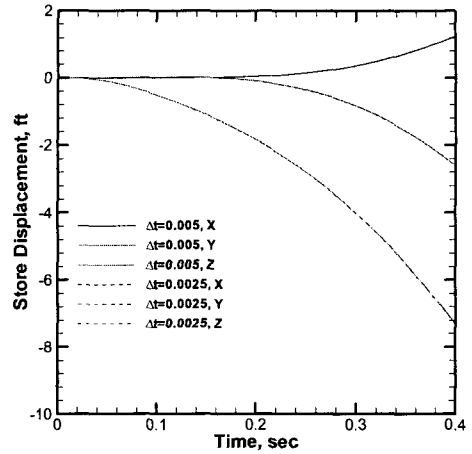
Fig. 10 Time step size study;
