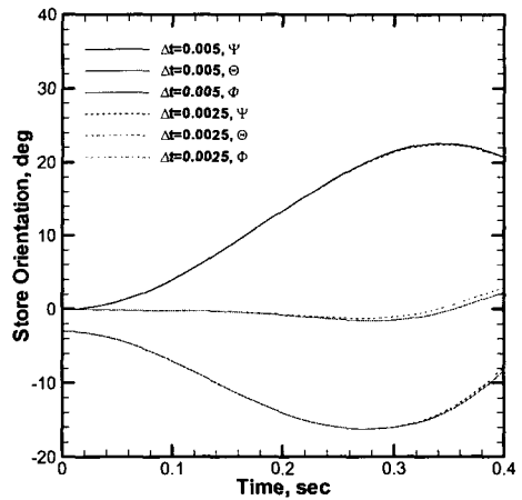
Fig. 11 Time step size study; Store orientation
