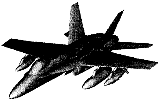
Fig. 2 Surface definition of F/A-18C and JDAM
