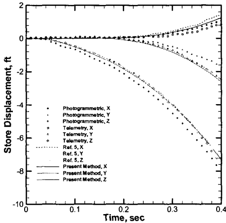
Fig. 5 Store displacement (case 2)
