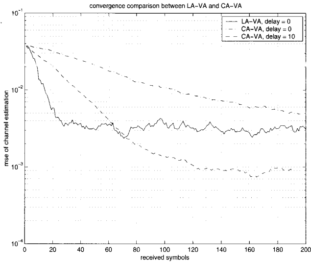
Fig. 3. Comparison between the LPA-VA and CA-VA with delay = 0, 10 for channel b estimation and updating. SNR is 13 dB.
