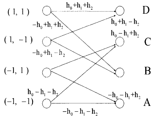
Fig. 2. The trellis for M=2 and L=2 . Branch values are determined by the channel response.
