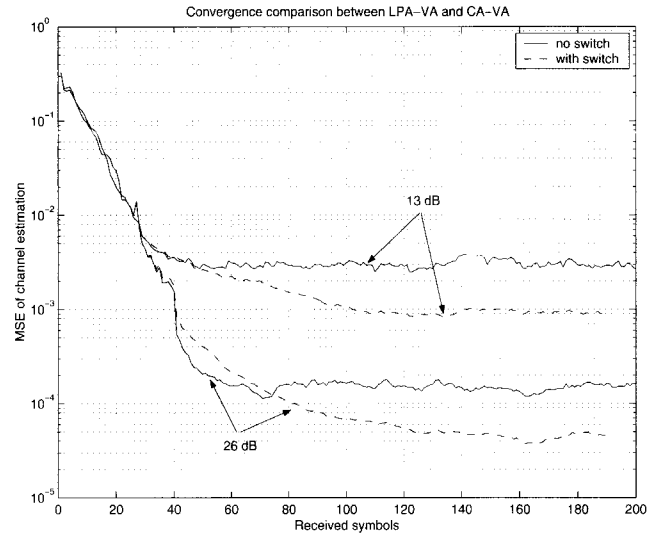
Fig. 4. Comparison between the proposed approach and the one that only uses LPA-VA with 4 survivors/state for channel b . SNRs are 13dB and 26dB, respectively. Average switch point for 13dB is the 49^{th} symbol, while that for 26dB is the 31^{th} symbol.
