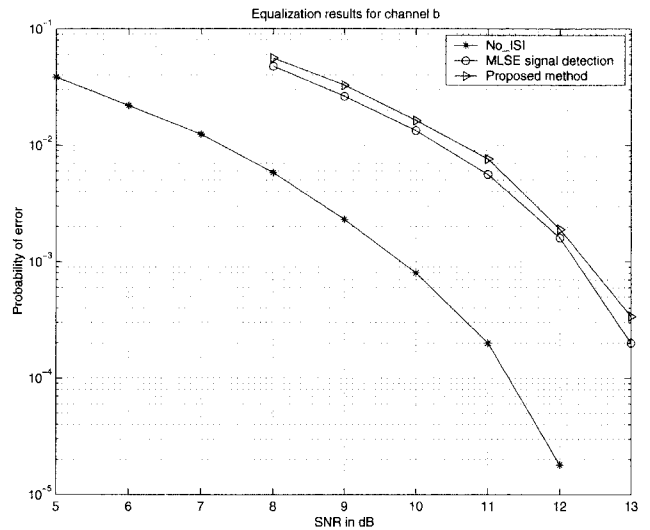
Fig. 7. Equalization result of the proposed approach for channel b .
