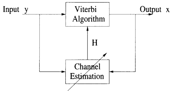
Fig. 1. L based channel estimation and signal detection. Three functions include initial channel estimation, signal detection, and decision feedback for channel updating.
