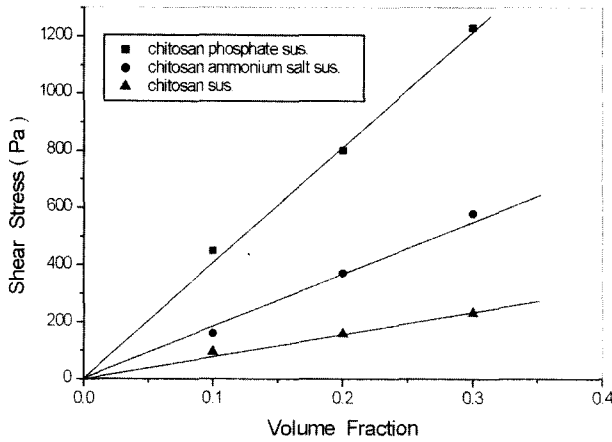
Fig. 4. Shear stress vs volume fraction for chitosan derivative suspensions ( E = 3 \text{ kV/mm} , \dot{\gamma} = 2 \text{ s}^{-1} ).
