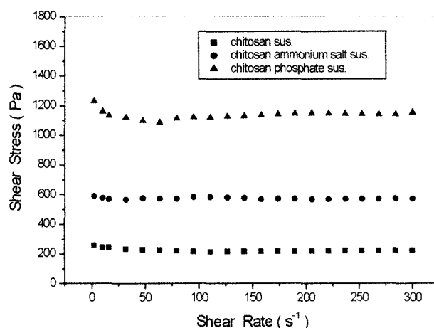
Fig. 2. Shear stress vs shear rate for chitosan derivative suspensions ( \phi = 0.3 , E = 3 KV/mm).
