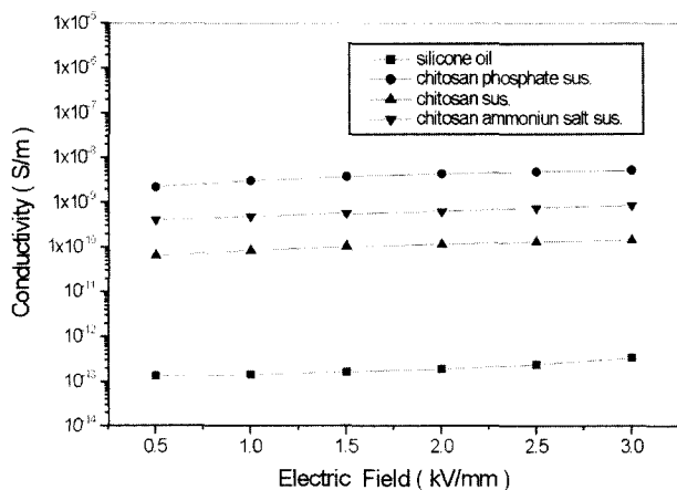
Fig. 1. Effect of electric field on conductivity for silicone oil and chitosan derivative suspensions.
