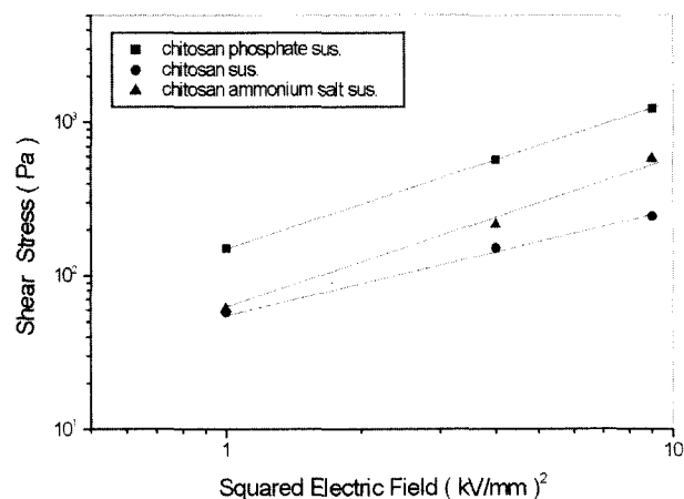
Fig. 3. Shear stress vs squared electric field for chitosan derivative suspension ( \phi = 0.3 , \dot{\gamma} = 2 s^{-1} ).
