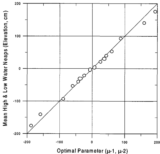
Fig. 3. Scatter plot of the \mu_1, \mu_2 parameters and HWONT, LWONT.
