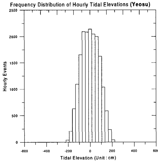
Fig. 1. Frequency diagram of the Tidal elevation data.
