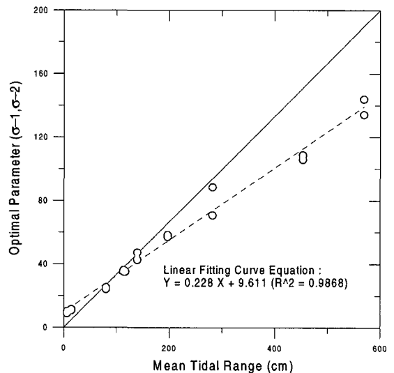
Fig. 4. Regression Curve of the \sigma_1, \sigma_2 parameters and mean range.
