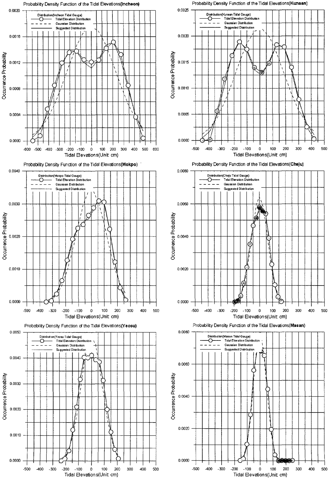
Fig. 2. Comparison of the normal and double-peak normal distribution function.
