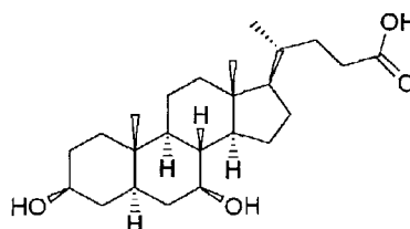
Fig. 1. Chemical structure of Ursodeoxycholic Acid
