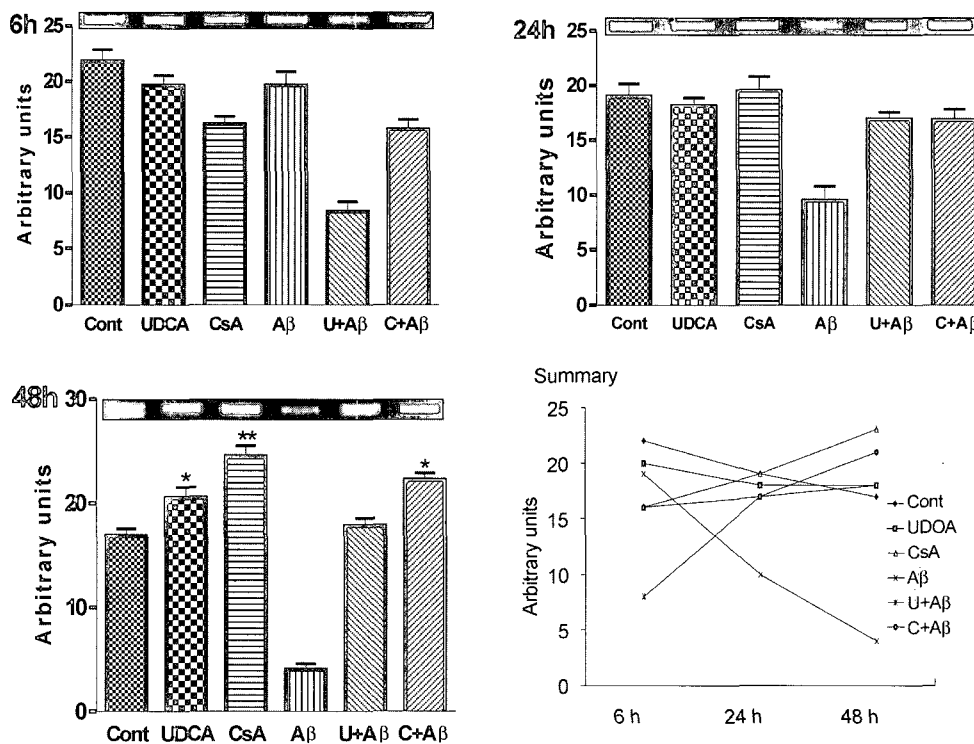
Fig. 3. Expression of A20 mRNA after treatment with different samples, UDCA, cyclosporine-A, A \beta 42, and co-treatment with A \beta 42 in the presence of UDCA or cyclosporine-A. A significant increase of A20 mRNA was detected from 48 h compared to control, whereas A \beta 42-treated group was dramatically decreased in a time dependent manner. Patterns of mRNA expression are shown in the summary figure. A20 mRNA was detected by using reverse transcription (RT)-PCR. The data represent means \pm SD of three determinations. *, p < 0.05 ; **, p < 0.001 .
