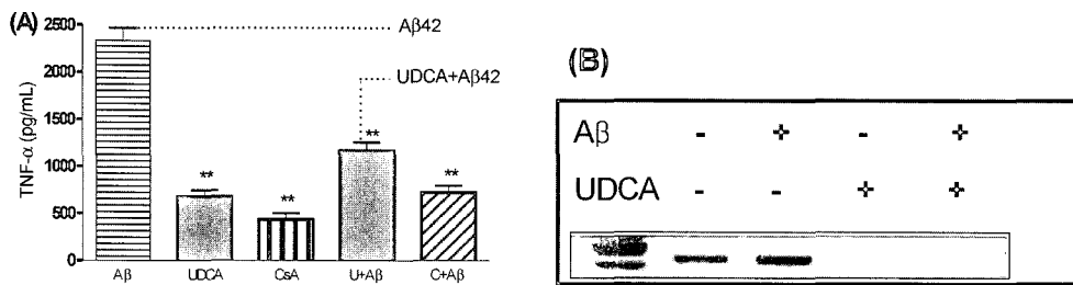
Fig. 2. Production of TNF- \alpha from different treatments in BV-2. TNF- \alpha protein level was determined by ELISA (A), and the expression of TNF- \alpha gene was observed by RT-PCR method to confirm the suppressive effect on TNF- \alpha (B). Final assays were done at 24 h. 100 \mu g/mL UDCA; 5 \mu g/mL cyclosporine-A; 5 \mu g/mL A \beta 42. Averages of triplicates \pm SD are shown and statistical significances were confirmed by Dunnetts Multiple Comparison Test vs. A \beta group. **, p < 0.01 .
