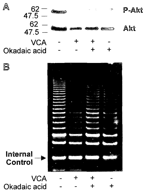
Fig. 7. Effects of protein phosphatase inhibitor on the VCA-induced dephosphorylation of Akt (A) and on the VCA-induced inhibition of telomerase activity (B). A253 cells were pretreated with okadaic acid and 10 ng/mL VCA or treated with either VCA or okadaic acid alone for 48 h. (A) Levels of Akt phosphorylation were determined by Western blot analysis using either total Akt and phospho-Akt antibodies. (B) Telomerase activity assessed by the TRAP assay. The figure is representative of three independent experiments.
