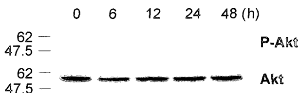
Fig. 5. VCA induces a time-dependent decrease in Akt phosphorylation in A253 cells. Cells were incubated for 24 h in 10% serum condition following by treatment 10 ng/mL VCA. Protein extracts were harvested, separated by SDS-PAGE and subjected to Western blot analysis using either total Akt and phospho-Akt antibodies.
