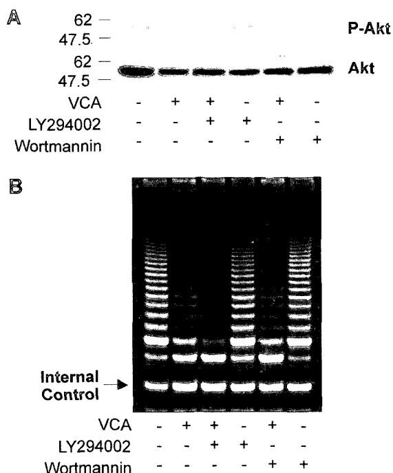
Fig. 6. Effects of PI3K inhibitors on the VCA-induced dephosphorylation of Akt (A) and on the VCA-induced inhibition of telomerase activity (B). (A) Levels of Akt phosphorylation were determined by Western blot analysis using either total Akt and phospho-Akt antibodies. (B) Telomerase activity assessed by the TRAP assay. The figure is representative of three independent experiments.
