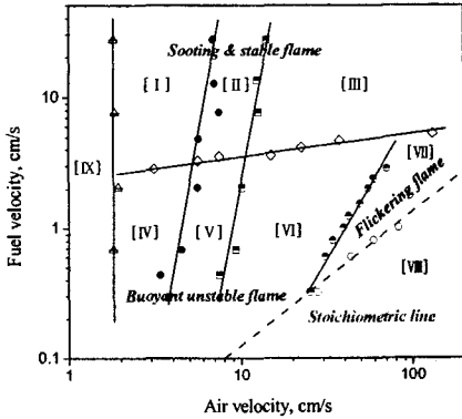
Fig. 2 Map of flame types of ethene/air IDF. Type I-III are stable and Type IV-VIII are unstable flames
