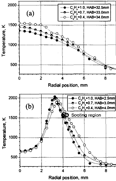
Fig. 6 Temperature profiles of IDF operated at three different ethene concentrations: (a) top of flames, and (b) soot inception zone
