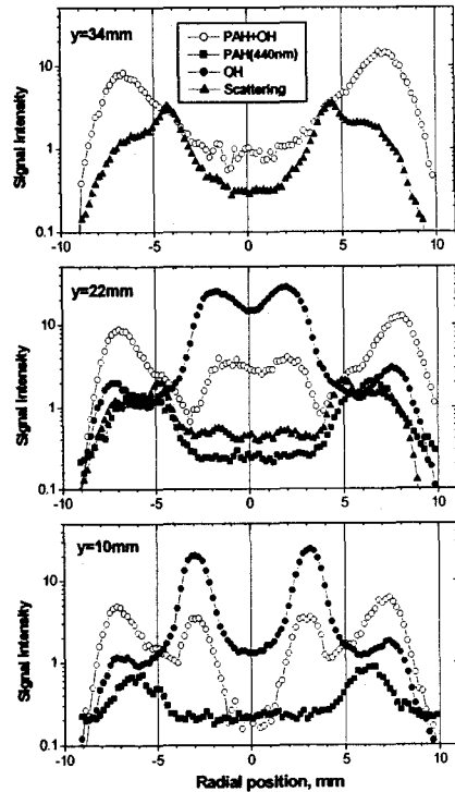
Fig. 3 A direct IDF picture, and corresponding (a) OH, (b) OH+PAH, (c) PAH by LIF, and (d) scattering images and signals at three different locations
