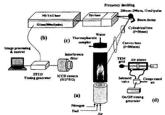
Fig. 1 Schematic diagram of the experiments: (a) IDF burner, (b) laser system diagnostics, (c) thermophoretic sampler, and (d) TEM grid system
