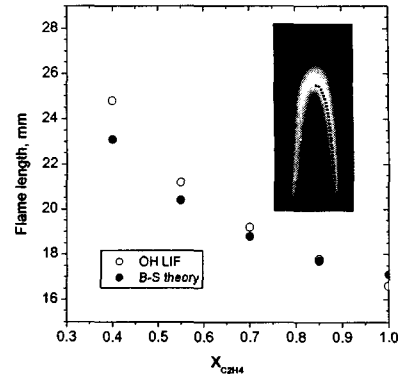
Fig. 5 Flame heights measured from OH LIF images and calculated from Burk- Shumann theory in the diluted ethene IDF. The inset illustrates OH image with predicted flame shape for X C 2 H 4 =0.7
