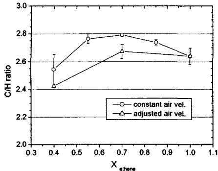
Fig. 8 Carbon to hydrogen molar ratios with different ethene concentrations in the fuel stream. One is measured in constant air velocity, but the other is collected in the adjusted air velocity to produce a flame height as same as that of X_{C_2H_4} = 1.0
