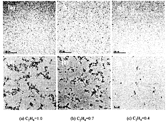
Fig. 7 TEM images of soot sampled from base of yellow flame (a-c) and from exhaust of IDF (d-f) according to fuel dilution ratios
