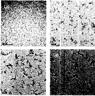
Fig. 4 TEM micrographs of soot particles along the sooting line at (a) flame base (HAB=2.5mm, Radius=4.5mm), (b) tip of OH radical (HAB=15mm, Radius=4.1mm), and far downstream ((c) HAB=25mm, Radius=3.4mm, (d) HAB=45mm, Radius= 2.8mm)
