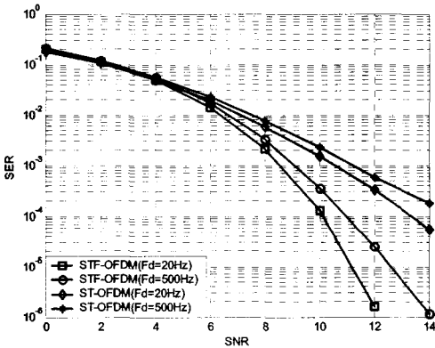
(a) QPSK
