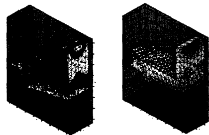
(b) t=23.3 sec
