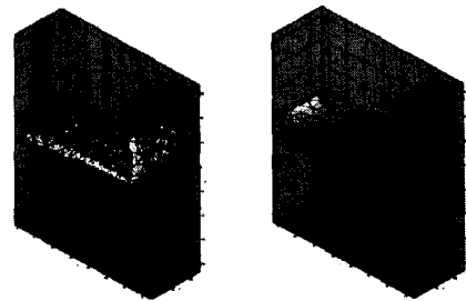
(a) t=2.4 sec
