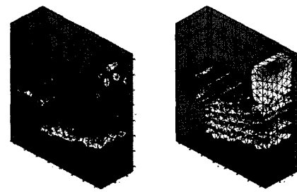
(c) t=128 sec
