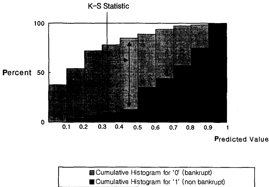
<Figure 1> K-S Statistic
