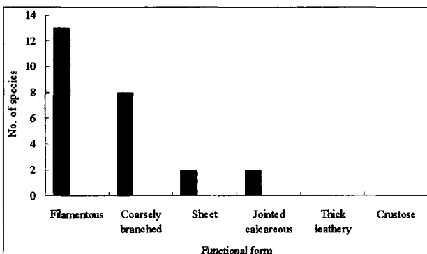
Fig. 1. Species number of six functional forms of the epiphytes occurring on Sargassum thunbergii .
