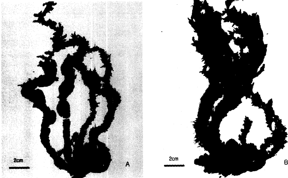
Fig. 2. Epiphytic marine alga ( Leathesia difformis ) at Norusum (A) and animal ( Mytilus edulis ) at Yeohangdo on the fronds of Sargassum thunbergii (B).
