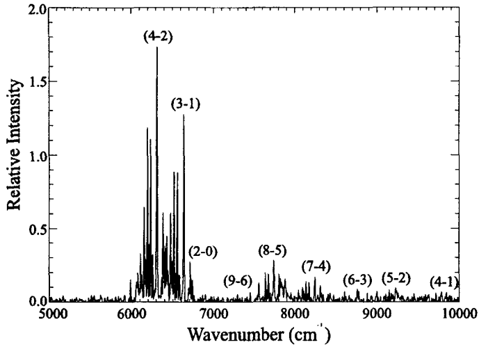
Figure 1. A sample of nighttime OH spectrum recorded at Esrange. Interferograms over about a 5-minute period (50 interferograms) were co-added to get this spectrum.
