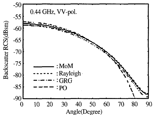
Fig. 3. Comparisons of analytical and numerical backscatter cross sections of a leaf at 0.44 GHz and VV-polarization.
