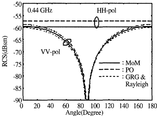
Fig. 5. Comparisons of analytical and numerical forward-scatter cross sections of a leaf at 0.44 GHz.
