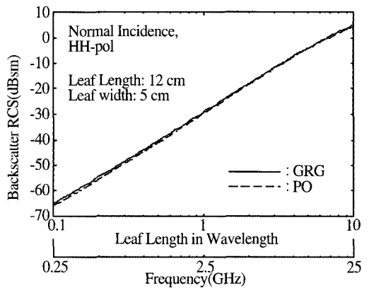
Fig. 6. Variation of the backscatter RCS of a leaf as a function of frequency at normal incidence.
