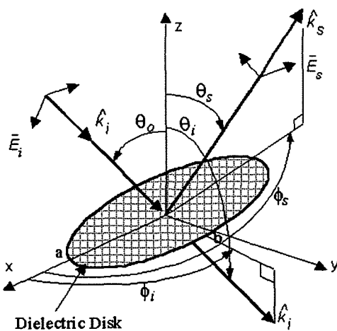
Fig. 1. Geometry of the scattering problem.
