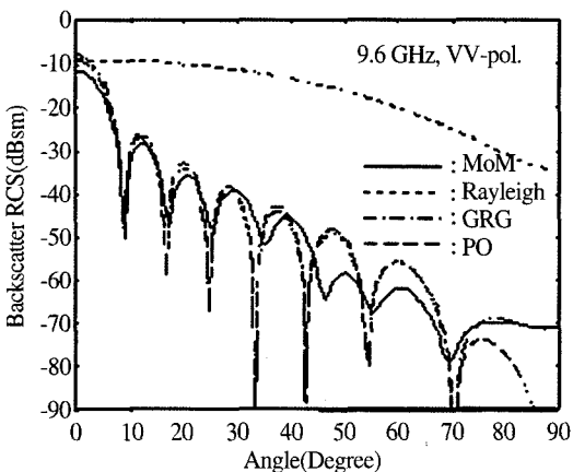
Fig. 2. Comparisons of analytical and numerical backscatter cross sections of a leaf at 9.6 GHz and VV-polarization.
