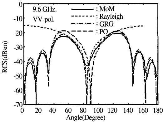
Fig. 4. Comparisons of analytical and numerical forward-scatter cross sections of a leaf at 9.6 GHz and VV-polarization.
