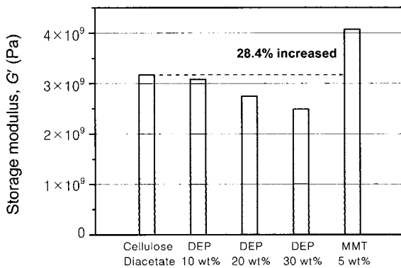
Figure 2. Glassy-state storage modulus of cellulose diacetate (CA), CA/DEP and CA/MMT systems measured at 50 °C and 1 Hz.
