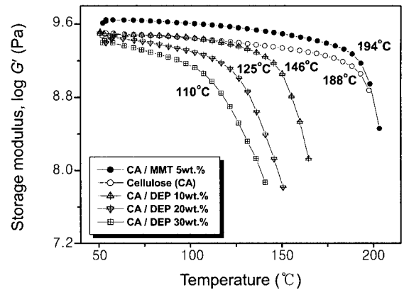
Figure 3. Storage modulus of cellulose diacetate (CA), CA/DEP and CA/MMT systems plotted as a function of temperature.
