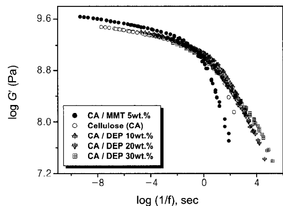
Figure 4. Storage modulus master curves for cellulose diacetate (CA), CA/DEP and CA/MMT systems using T_{GL} appearing in Figure 3.
