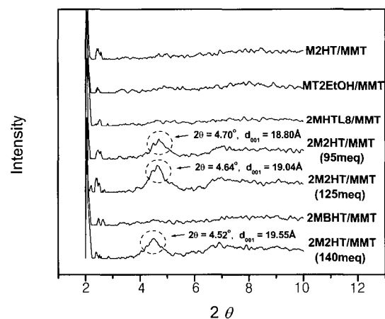
Figure 1. Wide angle X-ray diffractograms of cellulose nanocomposites containing different intercalants.
