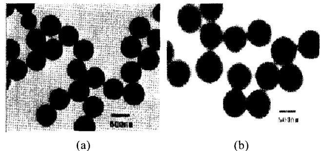
Figure 11. TEM micrograph of PVAc (a) and PVAc-PBA (b).
