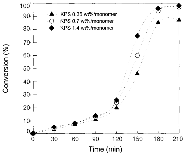
Figure 3. The variation of conversion with time for initiator concentration at PVAc-PBA copolymerization.
