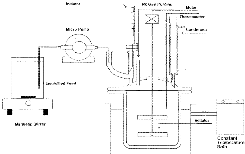
Figure 1. Experimental apparatus for VAc-BA copolymer emulsion polymerization.
