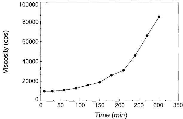
Figure 9. The variation of viscosity in PVAc-PBA copolymerization.
