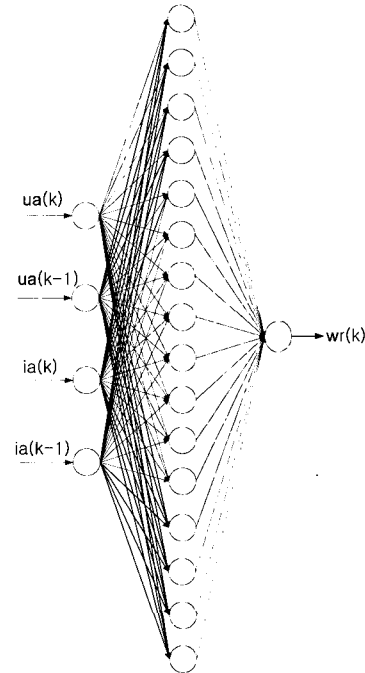
Fig. 3 Speed estimator by neural network
