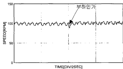
Fig. 12 Experimental response for step change of load torque. (0→1[N·m])
