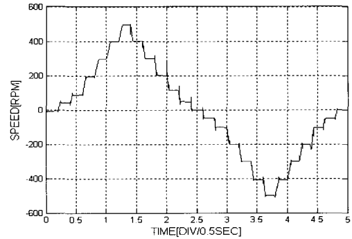
Fig. 6 Speed response of neural network estimator
