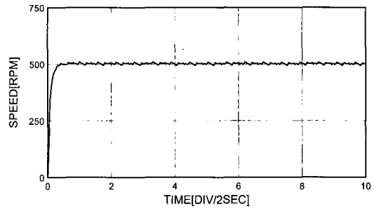
Fig. 10 Experimental response for step change of speed setting. (0→500[rpm])
