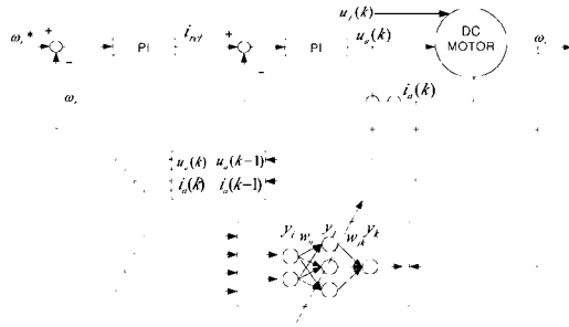
Fig. 5 Block diagram for training of neural network speed estimator
