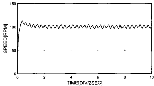
Fig. 8 Experimental response for step change of speed setting. (0→100[rpm])
