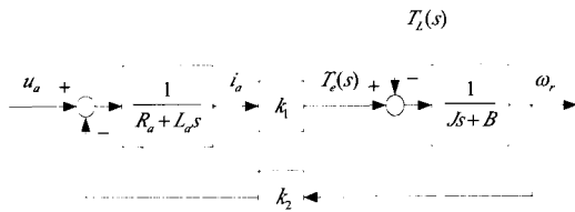
Fig. 2 System block diagram of DC motor
