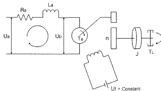
Fig. 1 Separate excitation field DC motor
