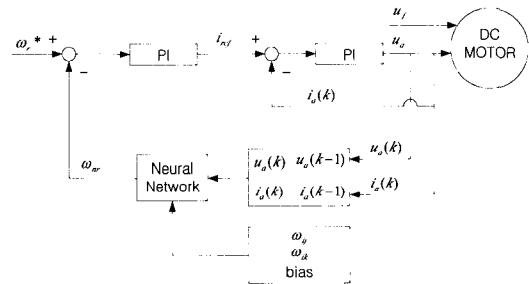
Fig. 7 Block diagram of speed control system by neural network
