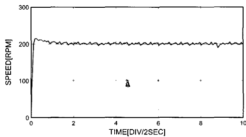
Fig. 9 Experimental response for step change of speed setting. (0→200[rpm])
