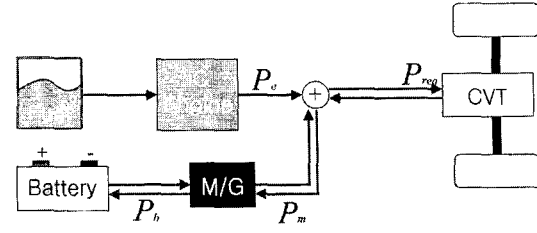
Fig. 3 Power flow of HEV
