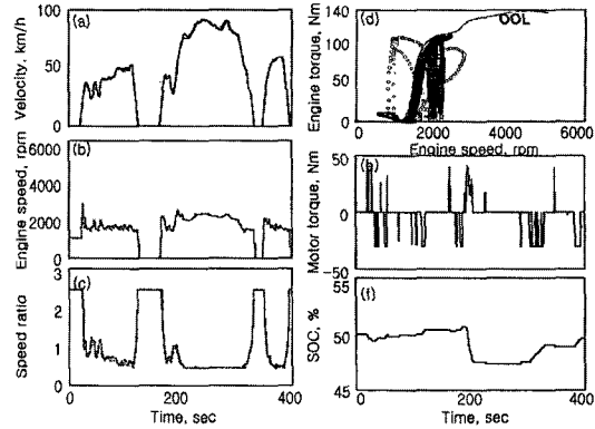
Fig. 7 Simulation results for equivalent fuel algorithm
