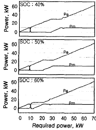
Fig. 5 Power distribution for equivalent fuel algorithm
