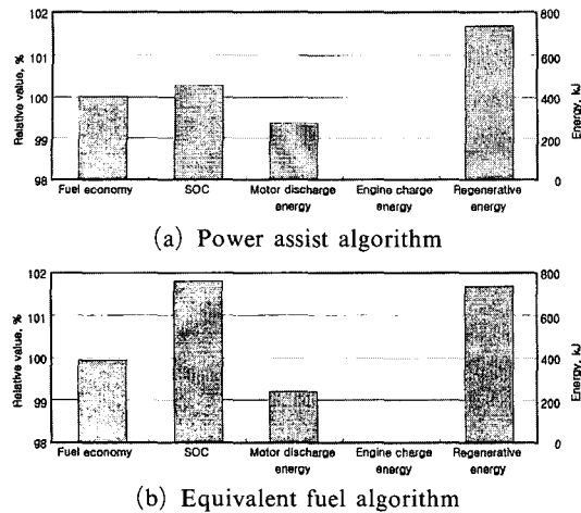
Fig. 8 Comparison of HEV performance
