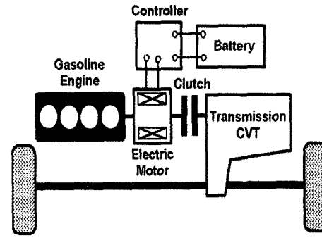
Fig. 1 Schematic diagram of parallel HEV
