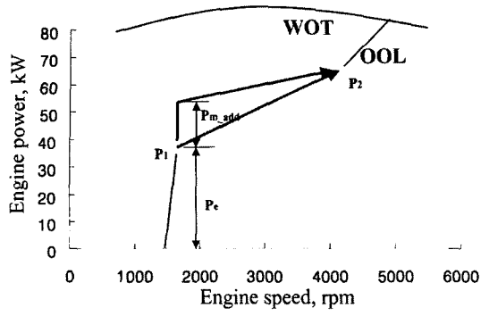
Fig. 2 Control strategy for power assist algorithm
