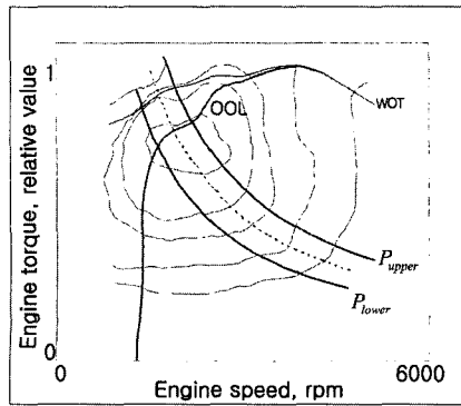
Fig. 4 Engine map
