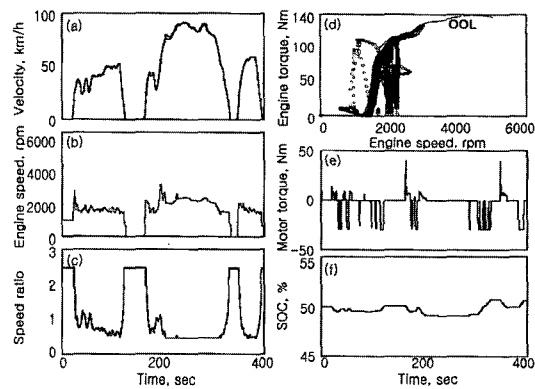
Fig. 6 Simulation results for power assist algorithm
