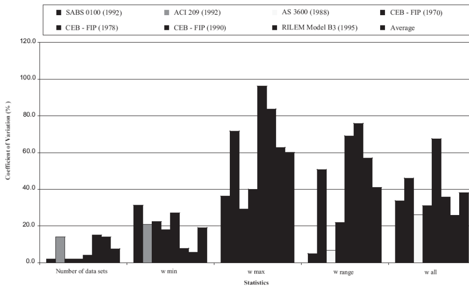
Fig. 1 Statistics pertaining to coefficients of variation.
