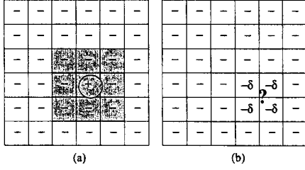
그림 2: Identification of droplets: (a) Apparent droplet, (b) Unapparent droplet. In (b), \delta is a small positive value such that \delta < \varepsilon
