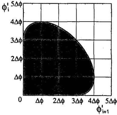
그림 8: Plot of (\phi'_i, \phi'_{i+1}) : the shaded region guarantees monotonic profiles in the case of \Delta\phi \geq 0
