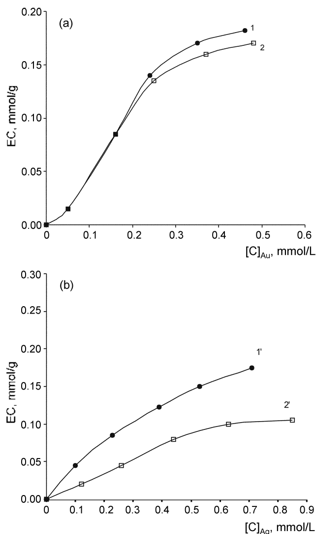
Figure 1. Isotherms of sorption of thiocyanate gold (a) and silver (b) complexes on anion exchanger AN-25 at pH = 2. 1,1' individual complexes. 2,2' simultaneous presence of gold and silver complexes.
