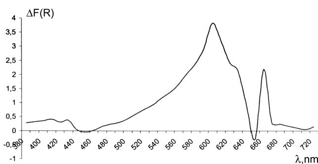
Figure 4. Diffuse reflection spectrum of gold (III) compound with tin (II) chloride in the phase of anion exchanger AN-25. The initial concentration of thiocyanate gold (III) complexes is 0.08 mmol/l; pH = 2.
