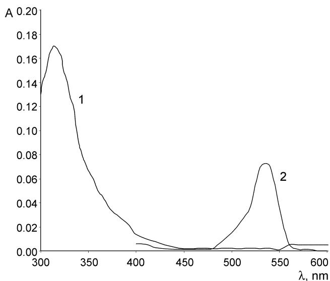
Figure 3. Absorption spectra of thiocyanate gold (III) complexes (1) and of gold (III) compound with SnCl 2 (2) in solution. The initial concentration of thiocyanate gold (III) complexes is 0.08 mmol/l; pH = 2.
