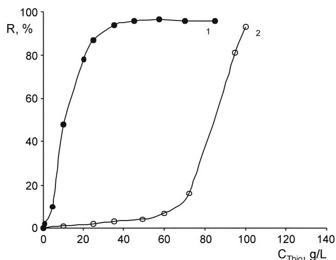
Figure 2. Desorption of silver (1) and gold (2) from anion exchanger AN-25 in dependence on thiocarbamide concentration in 0.3 M H 2 SO 4 . The initial concentrations during sorption are 0.33 mmol/L and 0.35 mmol/L for gold and silver, respectively.
