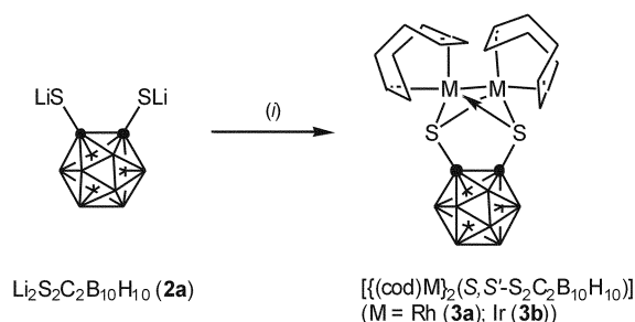
Scheme 2. Synthesis of the S,S' -chelating dinuclear metal(cod) complexes. Legend: (i) [\text{M}(\mu\text{-Cl})(\text{cod})]_2 (M = Rh, Ir), THF, 25^\circ\text{C} .
