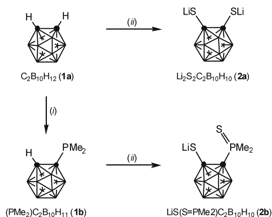
Scheme 1. Synthesis of the S,S' -chelating ligand 2 . Legend: (i) (a) \text{LiBu}^t , THF, -78^\circ\text{C} ; (b) \text{PMe}_2\text{Cl} , THF, 25^\circ\text{C} ; (ii) (a) \text{LiBu}^t , THF, -78^\circ\text{C} ; (b) \text{S}_8 , THF, 25^\circ\text{C} .
