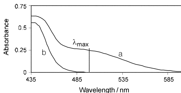
Figure 1. (a) The spectra of produced azo compound and (b) the blank solution against water. Conditions: nitrite ion, 0.8 \mu\text{g mL}^{-1} ; sulfuric acid, 1 \text{ mol L}^{-1} ; Triton X-100, 1.4% (v/v); p-nitroaniline, 0.02% (m/v); and diphenylamine, 0.05% (m/v). The blank solution was prepared in the same way except that distilled water was used instead of nitrite solution.
