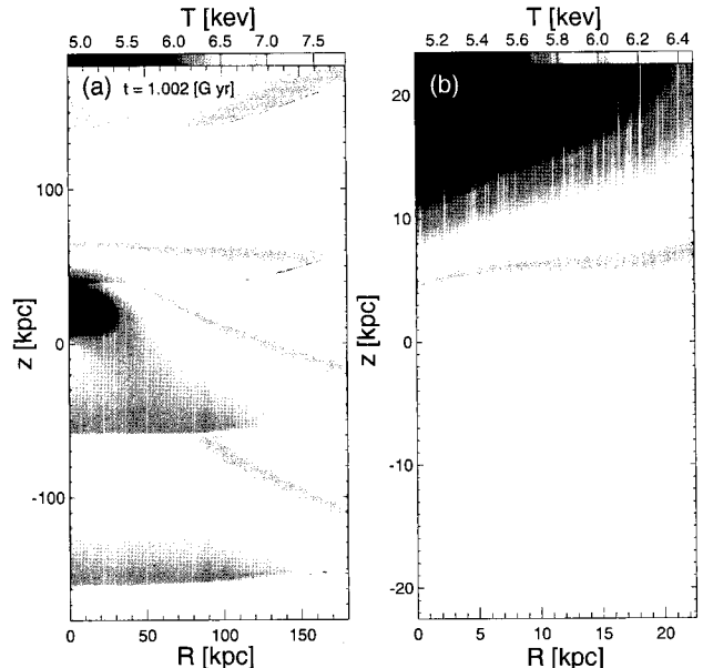
Fig. 1.— The temperature distribution of a cluster core at t = 1.0 Gyr. The periodic input waves are seen in Fig.1a as discontinuities that is nearly parallel to the R -axis. The waves propagate upward in these figures. (a) for z \lesssim 200 kpc, (b) for z \lesssim 20 kpc. Movies are available at http://th.nao.ac.jp/tsunami/index.htm .
