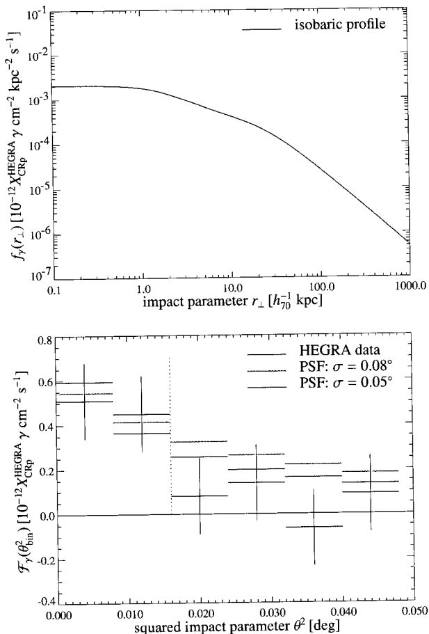
Fig. 3. — Upper panel: Modeled \gamma -ray surface flux profile of the cooling core region within the Virgo cluster. The profile is normalized by comparing the integrated \gamma -ray flux above 730 GeV to HEGRA data of M 87 within the innermost two data points. Lower panel: Comparison of detected to predicted \gamma -ray flux within the central aperture and the innermost annuli for two different widths of the PSF. The red lines correspond to an optimistic PSF of \sigma = 0.05^\circ whereas the green lines are calculated for a conservative \sigma = 0.08^\circ for a soft \gamma -ray spectrum. The vertical dashed line separates the data from the noise level at a position corresponding to r_\perp = 37.5 kpc.
