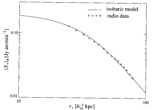
Fig. 5. — Radio emissivity profile of the Perseus mini-halo at 1.4 GHz observed by Pedlar et al. (1990) (crosses) and predicted due to hadronic interactions of CRp by Pfrommer & Enblin (2004a). Both the required CRp scaling ratio X_{\text{CRp}} \simeq 2\% and the morphological match of the observed and predicted radio emissivities strongly indicate the hadronic origin of radio mini-halos.
