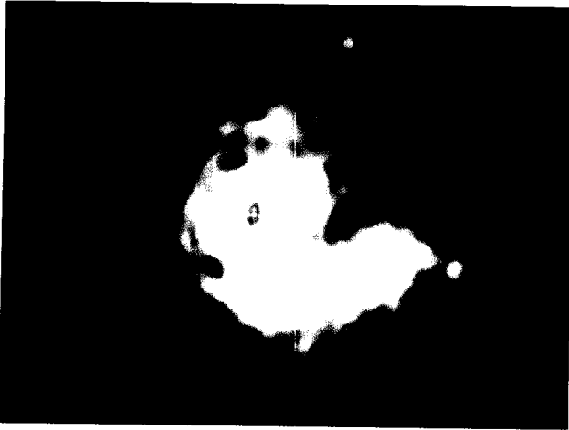
Fig. 4. — The Perseus radio mini-halo at 1.4 GHz from Pedlar et al. (1990) with an extent of 160 h_{70}^{-1} kpc in diameter. At the very center is an extremely bright flat-spectrum core owing to relativistic outflows of the radio galaxy NGC 1275. This outflow was subtracted from this image to make the extended structure more visible. The position of the radio galaxy is marked by the green cross in the center of the red region.
