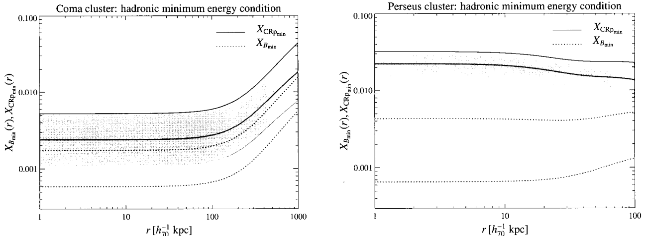
Fig. 6. — Profiles of the CRp-to-thermal energy density X_{\text{CRp, min}}(r) (solid) and magnetic-to-thermal energy density X_{B, \text{min}}(r) (dotted) as a function of deprojected radius are shown. The different energy densities are obtained by means of the hadronic minimum energy criterion. The left panel shows profiles of the Coma cluster while the right panel represents profiles of the Perseus cluster. The light shaded areas represent the logarithmic tolerance regions of X_{B, \text{min}}(r) and X_{\text{CRp, min}}(r) , respectively, while the dark shaded regions indicate the overlap and thus the possible equipartition regions in the quasi-optimal case.
