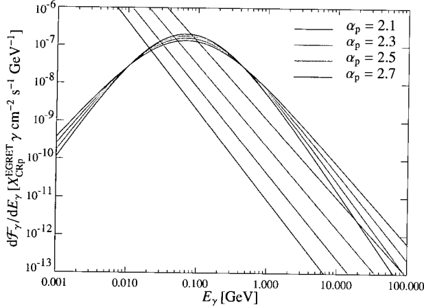
Fig. 1. — Theoretical \gamma -ray spectra of the Perseus cluster resulting from CRp hadronic interactions with the cooling core gas. The assumed CRp spectra are normalized to be marginally consistent with the EGRET E_\gamma > 100 MeV non-detection limits. Results for different proton spectral indices are shown. The \pi^0 -decay bump is clearly visible. Secondary CRs scatter cosmic microwave background photons into the \gamma -ray regime by the inverse Compton process. The resulting power-law emission dominates the low energy part of the spectrum. The CR population was calculated neglecting synchrotron radiation energy losses. Thus, realistic inverse Compton spectra due to this process will exhibit a lower normalization than displayed here.
