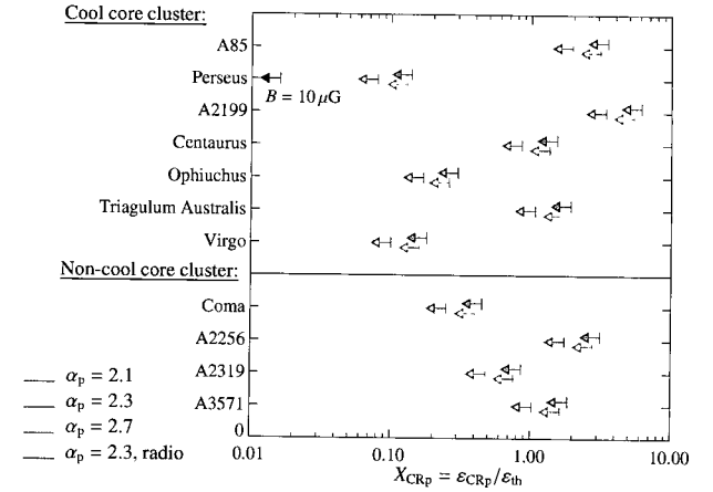
Fig. 2. — EGRET \gamma -ray constraints on the (central) CRp energy density ( \epsilon_{\text{CRp}} , for various CRp spectral indices) in terms of the cluster central thermal energy density ( \epsilon_{\text{th}} ) for cooling core and non-cooling core clusters. The constraint from the Perseus cluster radio mini-halo observation is also displayed while assuming a typical cooling core cluster magnetic field strength (blue arrow). If radio mini-halos are entirely produced hadronically by CRps then the constraint derived for the Perseus cluster is an actual measurement for X_{\text{CRp}} and not only an upper limit.
