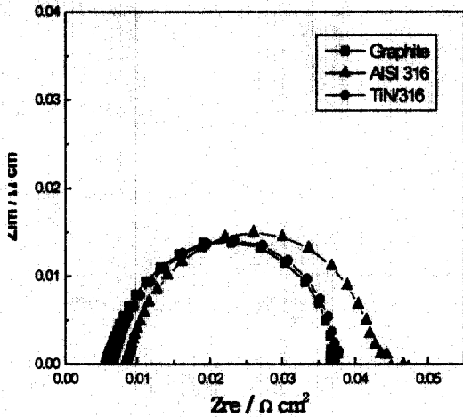
Fig. 4. Initial Nyquist plots for the single cells assembled with graphite, AISI 316, TiN/316 bipolar plates at a cell voltage = 0.85 V; operating temperature = 80 °C; operating pressure = 1 atm ; \lambda_{H_2} = 1.5 and \lambda_{O_2} = 3.
