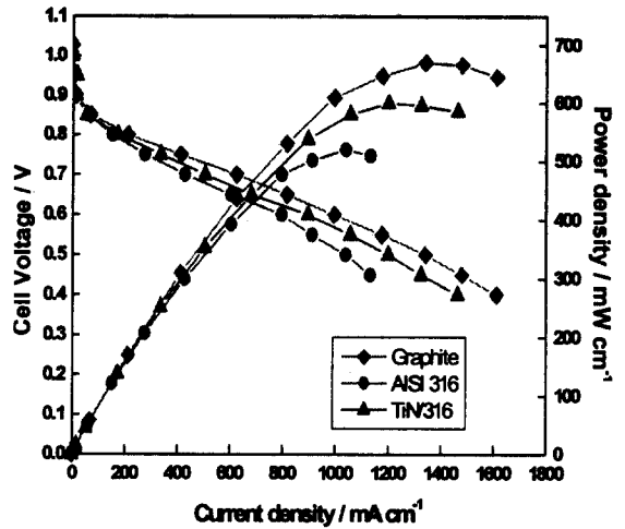
Fig. 3. i-V curves for the single cells using graphite, AISI 316, and TiN/316 bipolar plates; operating temperature = 80 °C operating pressure = 1 atm; \lambda_{H_2} = 1.5 and \lambda_{O_2} = 3 .
