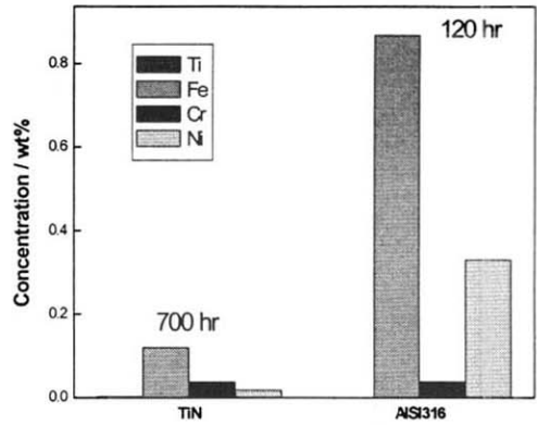
Fig. 7. Concentration of metal elements in the MEA assembled with AISI 316 and TiN/316 bipolar plates measured by ICP after the long-term operation.
