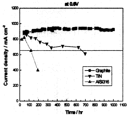
Fig. 5. Current density measured at a cell voltage of 0.6V during the long-term operation for the single cells assembled with graphite, AISI316, and TiN/316 bipolar plates; operating temperature = 80 °C; operating pressure = 1atm; \lambda_{H_2} = 1.5 and \lambda_{O_2} = 3.
