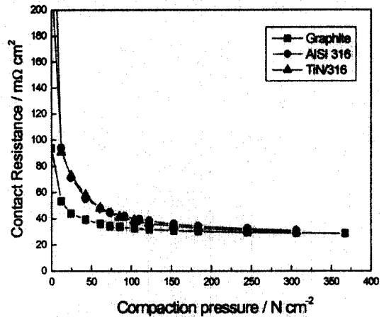
Fig. 1. Contact resistance of graphite, AISI316, and TiN-coated 316 plates measured at various compaction pressures.
