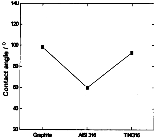
Fig. 2. Static water contact angle of graphite, AISI 316, and TiN/316 plates.
