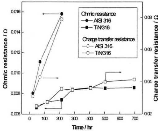
Fig. 6. Ohmic and charge transfer resistance during the long-term operation for the single cells assembled with graphite, AISI 316, and TiN/316 bipolar plates; operating temperature=80 °C; operating pressure=1 atm; λH2=1.5 and λO2=3.
