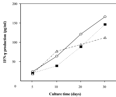
Figure 5. The concentration of IFN- \gamma according to the clonal expansion of CII (255~274)-reactive T cells in SFMC (○) and PBMC (■) from RA patient and PBMC from healthy control subject (△).
