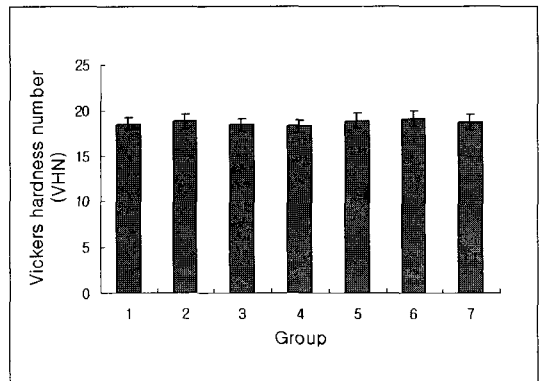
Fig. 4. Results of Vickers hardness test.
