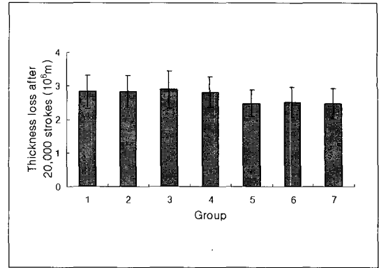
Fig. 6. Results of abrasion test using soap solution.
