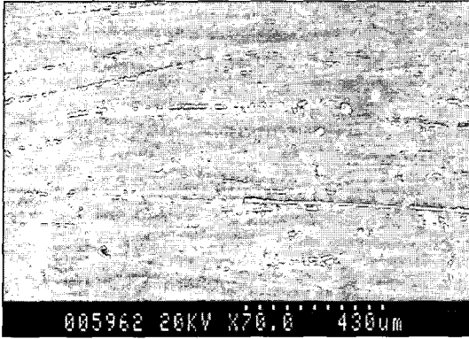
Fig. 17. Lucitone 199® : SEM photograph of abraded surface with soap solution at magnification of 70X.
