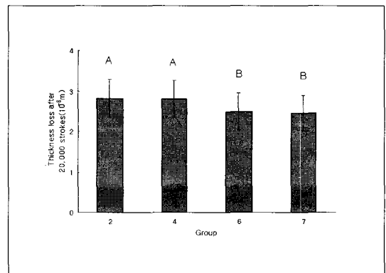
Fig. 10. Results of abrasion test in injection molding technique using soap solution (Mann-Whitney test). Between same characters, there are no significant difference at the 0.05 level.
