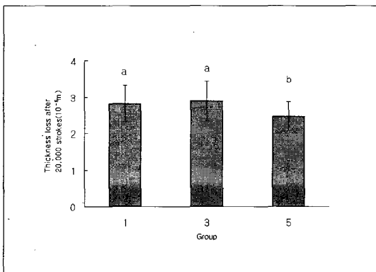
Fig. 9. Results of abrasion test in compression molding technique using soap solution (Mann-Whitney test). Between same characters, there are no significant difference at the 0.05 level.
