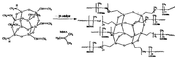
Fig. 1. The opening of the double chain of vinyl-POSS by platinum.
