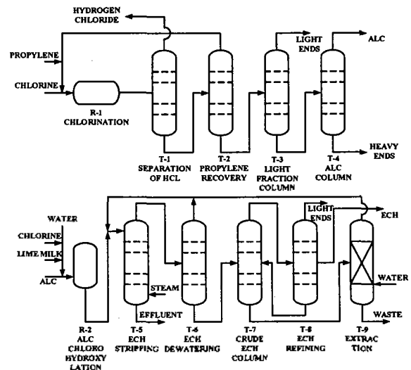
Fig. 5. ECH Process Flow Diagram.
