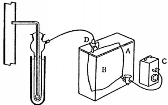
A: Sample case B: Sampling bag C: Vacuum pump D: Cock
