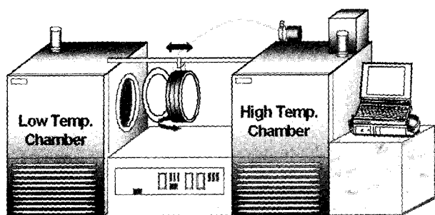
Figure 1. Human-Clothing-Environment simulator.
