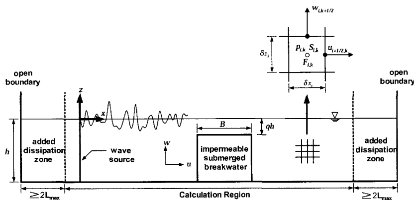
Fig. 1. Definition sketch of numerical wave flume.
