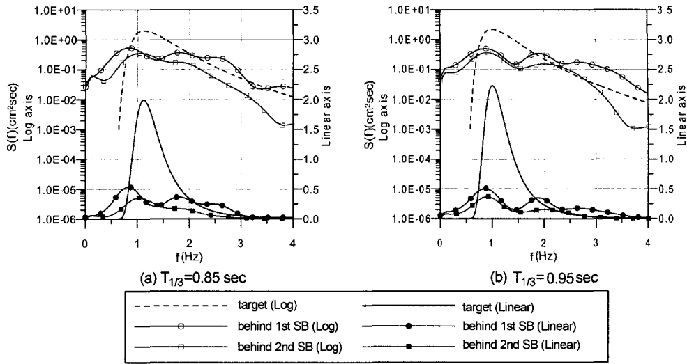
Fig. 5. Comparison of frequency spectrum for 1st ISB and 2nd ISB in Case3.
