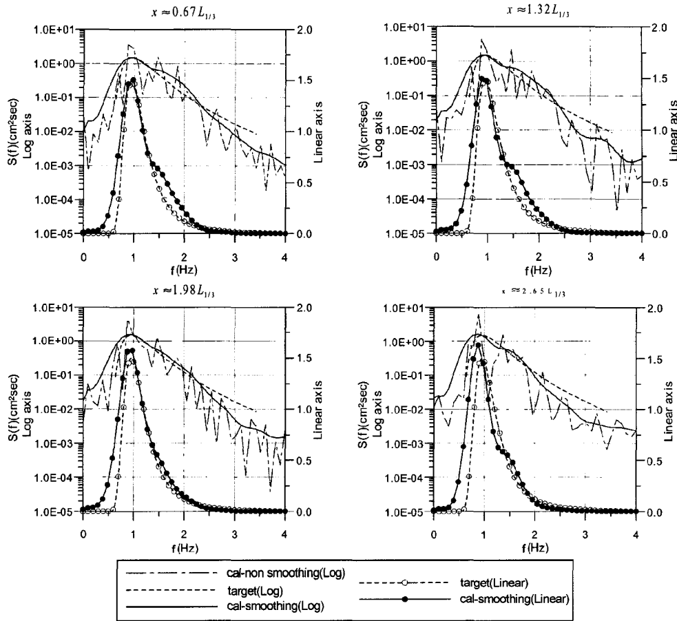
Fig. 3. Comparison of target spectrum and calculated spectrum at each point.
