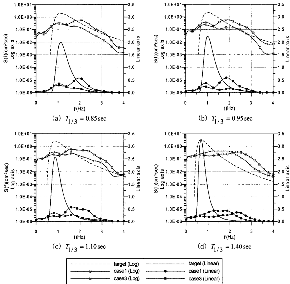
Fig. 4. Comparison of frequency spectrum for 1-row ISB and 2-row ISB at the rear of the structure.
