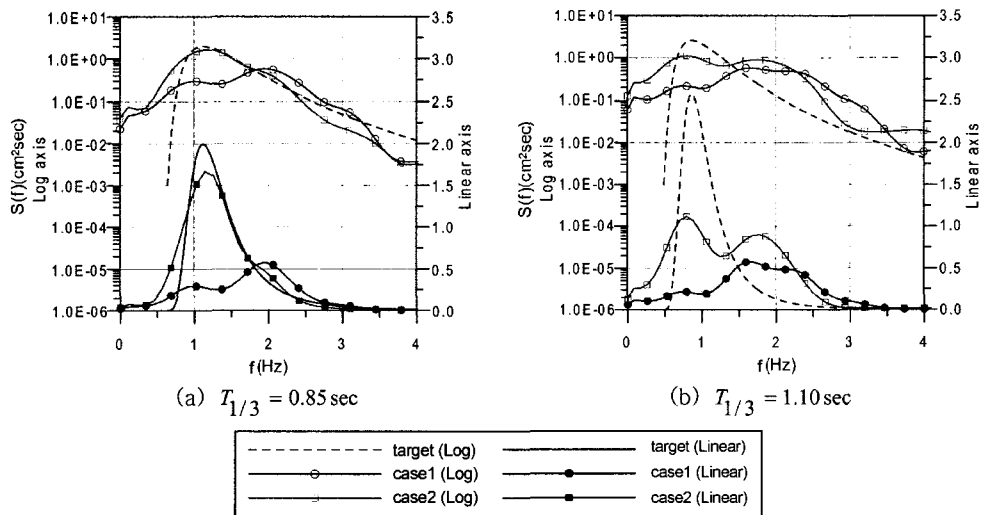
Fig. 6. Comparison of frequency spectrum for Case1 and Case2 at the rear of the structure.
