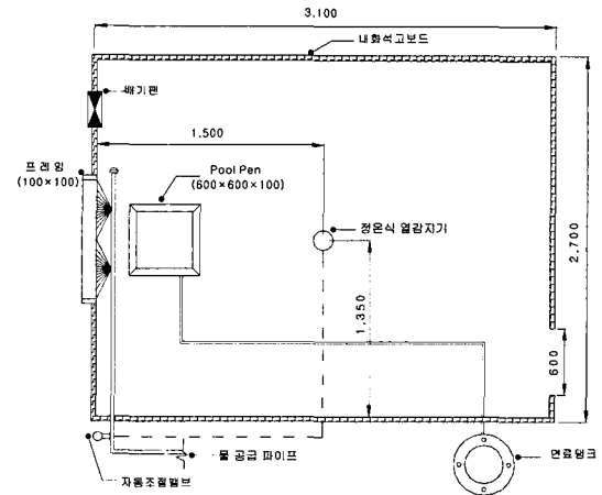
Fig. 2. Layout for experimental devices.
