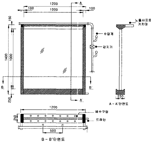
Fig. 1. Frame dwg. of water spray covered widow equipment.
