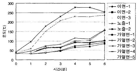
Fig. 11. Thermocouple temperature on both surfaces of ordinary glass.
