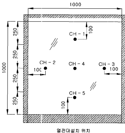
Fig. 3. Layout for thermocouple installation & ignition source.
