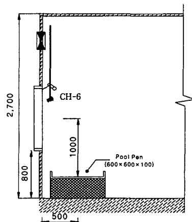
Fig. 2. Layout for experimental devices.
