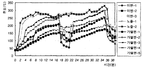
Fig. 10. Thermocouple temperature on both surfaces of tempered glass.
