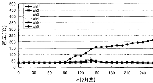
Fig. 12. Thermocouple temperature on glass surface after detection & water spray.
