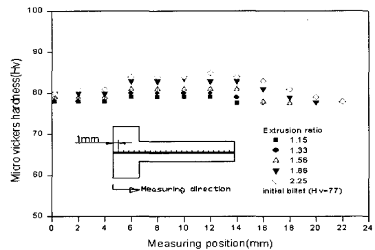
Fig. 5 Hardness distribution in the center line of a extruded pin(Al1050)
