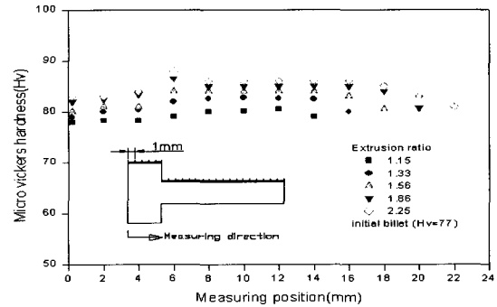
Fig. 4 Hardness distribution in the surface of a extruded pin(Al1050)
