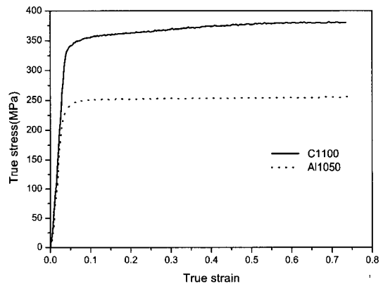
Fig. 1 True stress - strain curves of billets
