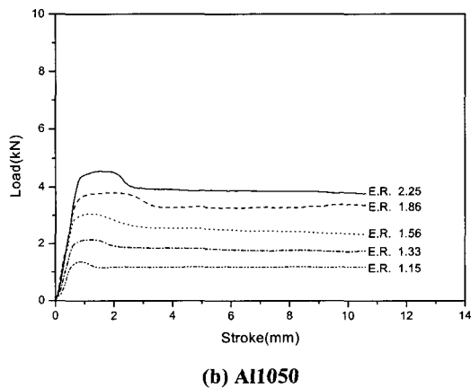
Fig. 3 Load - stroke curves according to extrusion ratios
