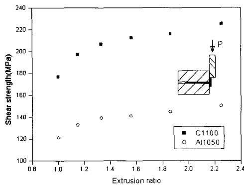
Fig. 7 Comparison of shear strength according to extrusion ratios
