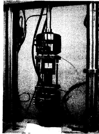
Fig. 2 Experimental set-up(MTS858)
