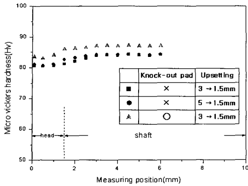
Fig. 6 Hardness distribution in the center line after upsetting(Al1050)
