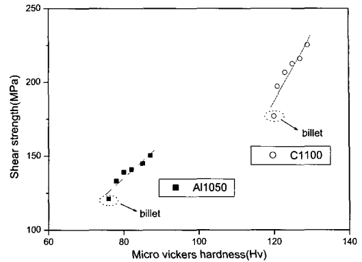
Fig. 8 Relationship between shear strength and hardness
