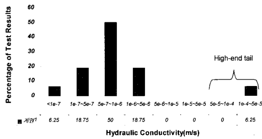
Fig. 7. Histogram of 18 packer-test results from Taejon LNG Pilot Cavern.
