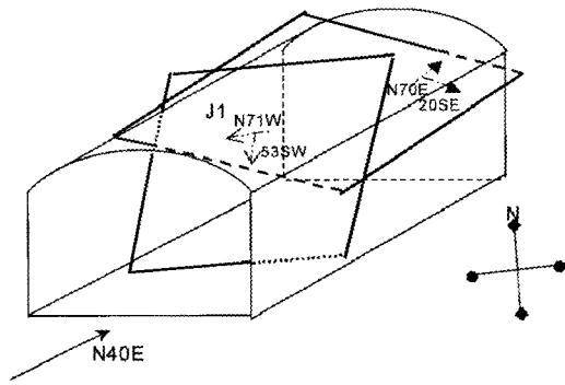
Fig. 3. Schematic diagram representing direction of Joint set 1 and a water carrying main joint.
