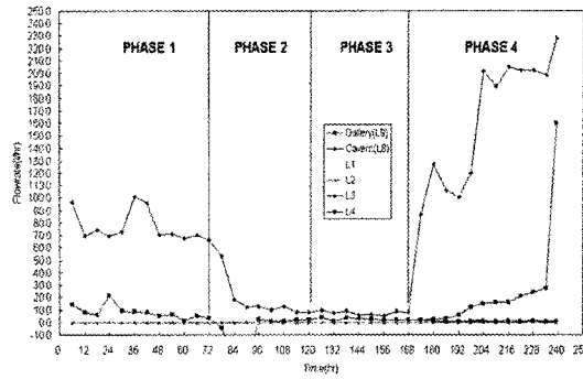
Fig. 4. Flow rate of Cavern and Leakage points inflows during the hydrogeological interference test between holes.
