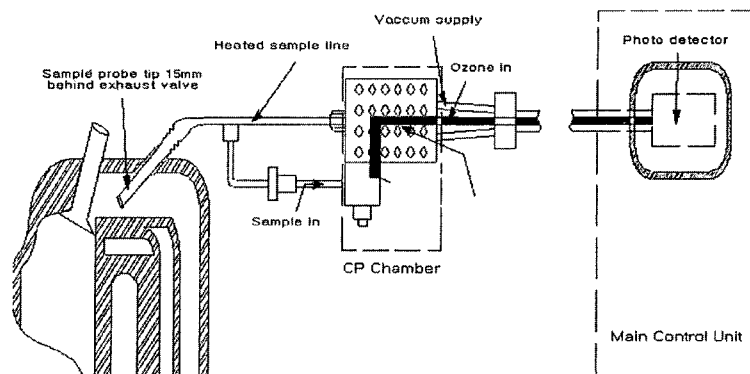
Fig. 2 Measurement system of NO emissions
