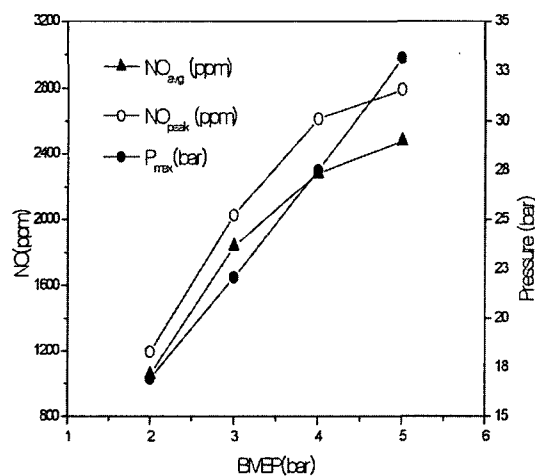
Fig. 7 NO emission and maximum combustion chamber pressure
