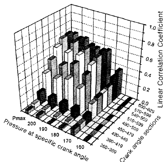
Fig. 6 Linear correlation coefficient between NO and pressures with respect to sampling crank angle sections
