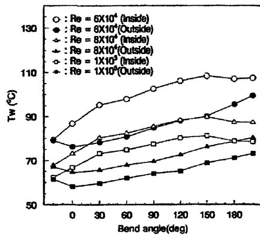
Fig. 11 Comparison of wall temperature profiles between inside and outside along 180^\circ bend for swirl of L/D=7 with respect to Re
