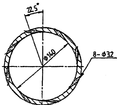
Fig. 4 Cross-section of the swirl generator
