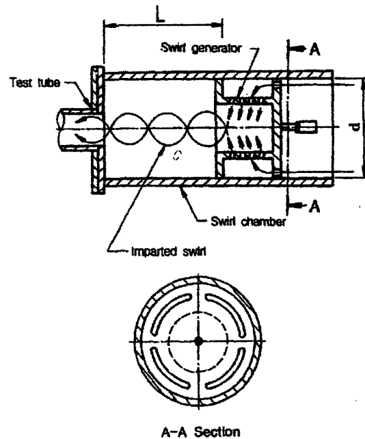
Fig. 3 Schematic diagram of inlet section
