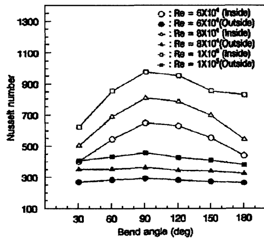
Fig. 22 Comparison of Nusselt number profiles along the 180^\circ bend for Re=6 \times 10^4
