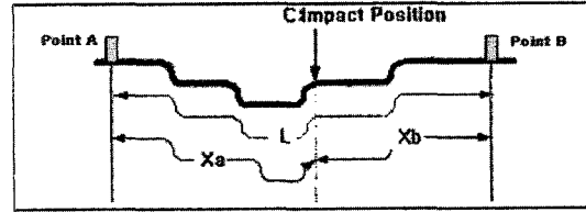
Fig. 2 Pipeline description
