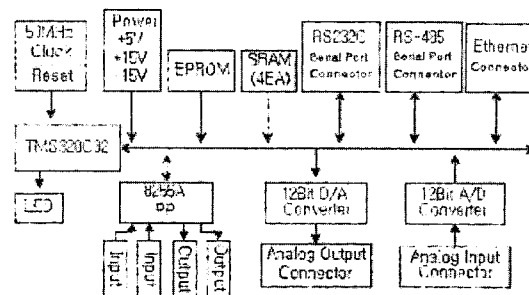
Fig. 4 Developed DSP TMS320C32 Board
