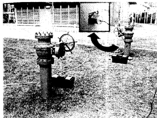
Fig. 7 Practical pipeline and impact detection sensors
