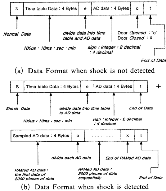
Fig. 5 Data format of monitoring S/W
