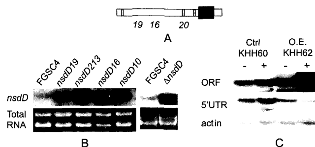
Fig. 2. Autoregulation of nsdD . (A) Schematic structure of nsdD ORF. Black box represents the zinc finger domain. Introns are indicated by small gray boxes. Figures represent mutation sites. (B) The nsdD transcript levels in allelic and ORF deleted mutants. Total RNA was extracted from 16 h cultured mycelia of nsdD allelic and deletion mutants and hybridized with a probe specific for nsdD ORF (left 5 lanes) or 5'UTR (right 2 lanes). nsdD213 and nsdD16 are the same alleles. (C) Effect of nsdD over-expression under the niiA promoter on the expression of nsdD by its own promoter. Total RNA was extracted from nsdD over-expressed strain (KHH62) and its isogenic control strain (KHH60) cultured for 16 h in MM broth containing 0.2% ammonium tartrate (-) or 0.6% sodium nitrate (+) as the sole nitrogen source, and Northern hybridized. The upper lane was probed with nsdD ORF and the middle lane with 5'UTR. When induced by sodium nitrate, the amount of nsdD transcript by the niiA promoter in KHH62 dramatically increased (upper, lane 4), while that by the nsdD promoter declined (middle, lane 4).
