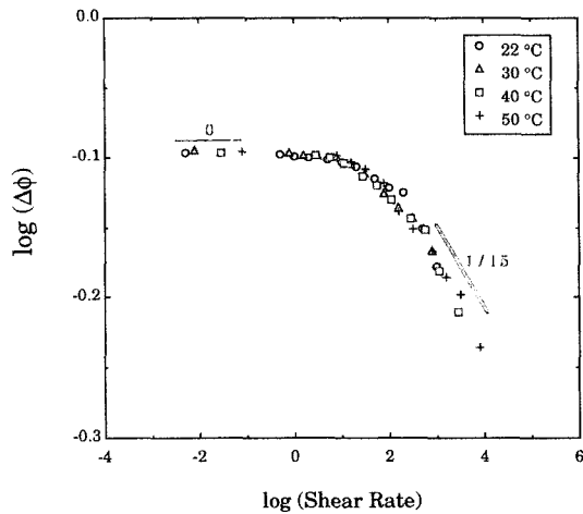
Figure 9. A master plot of \log \Delta\Phi(\dot{\gamma}, T) vs \log(\dot{\gamma}) .
