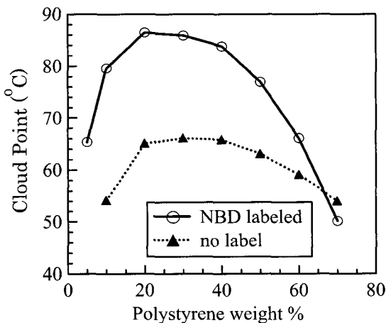
Figure 2. Phase diagram of NBD-PS/PB (50:50 by weight) in DOP.
