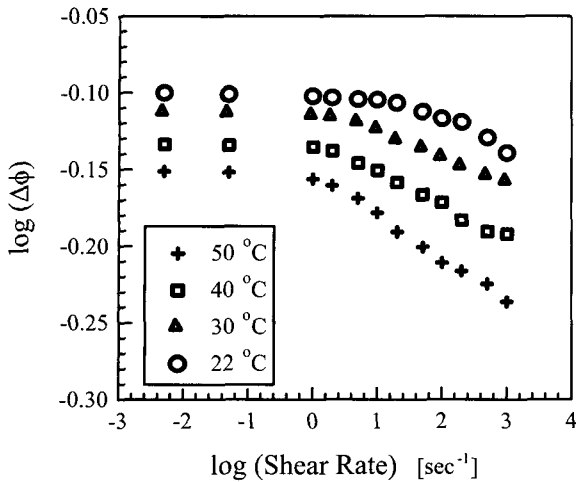
Figure 8. \Delta\Phi(\dot{\gamma}, T) as a function of shear rate for four different temperatures.
