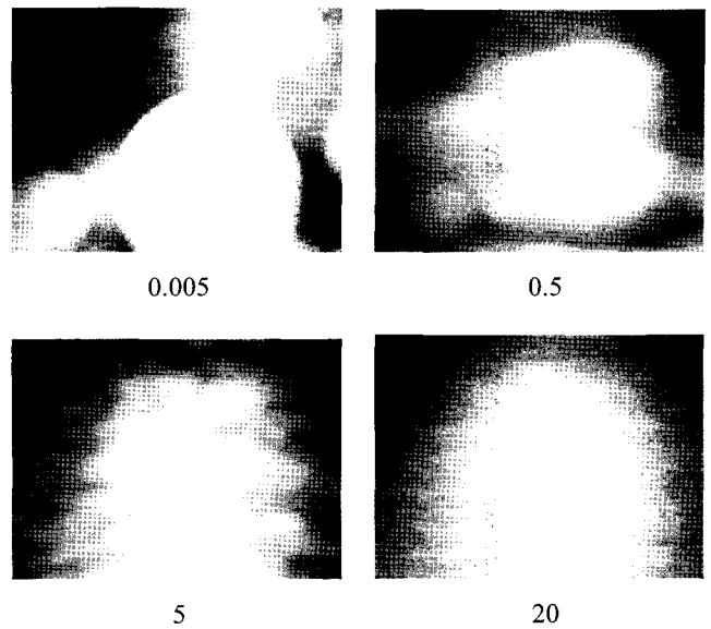
Figure 7. Microscopic images of 8 wt% 50:50 NBD-PS ( M_w=110000 ) / PB ( M_w=22000 ) in DOP at 50 °C at different shear rates. Quench depth is 27 K.
